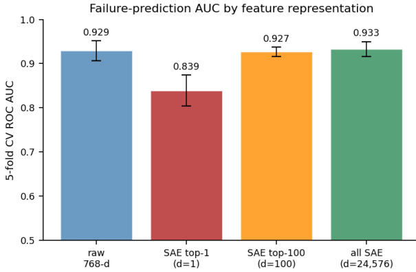
Fig. 6: Failure-prediction AUC under four feature representations (5-fold stratified CV, class-balanced logistic regression). The raw 768-dimensional residual stream matches the top-100 SAE features. The SAE basis is interpretable but not adding predictive power on this task at this layer.
