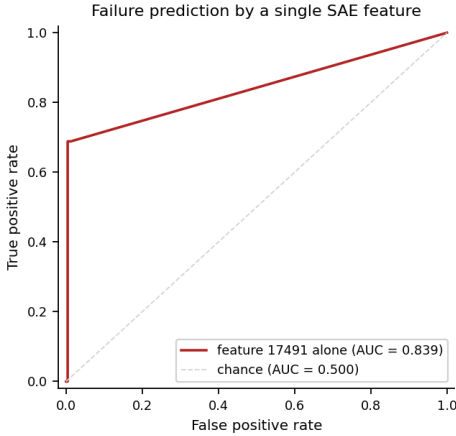
Fig. 8: ROC curve for predicting IOI failure from feature 17,491’s activation alone. AUC = 0.839. The raw residual stream reaches a higher AUC (0.929) without the SAE; we report this curve to show how much of the keys signal a single feature picks up.
