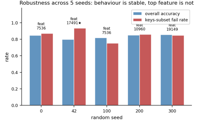
Fig. 7: Multi-seed robustness check ( n=5 seeds, 300 prompts each). The behavioural keys-failure rate is stable across seeds (75–93%, never below 75%). The headline SAE feature is not: 17,491 is the top- |d| feature in only the originally-reported seed. The other four seeds promote different features (7536 in two cases, 10960, 19149) to the top position. The star marks feature 17,491 where it appears.
