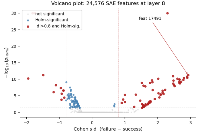
Fig. 2: Volcano plot of all 24,576 SAE features at layer 8. Each point is a feature; the x -axis is the Cohen’s d between the feature’s mean activation on failed trials and its mean on successful trials (positive = fires more on failure). The y -axis is -\log_{10}(p_{\text{Holm}}) from Welch’s t -test with Holm-Bonferroni correction across all features. Red points are both Holm-significant ( p < 0.05 ) and have a large effect size ( |d| > 0.8 ); the strongest predictor of failure (feature 17,491) is labelled.
