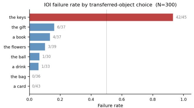
Fig. 4: IOI failure rate by transferred-object choice. Seven of the eight choices yield failure rates between 0.0% and 16.2%; the “the keys” subset (red) is at 93.3%. Numbers next to each bar show fail count / total.
