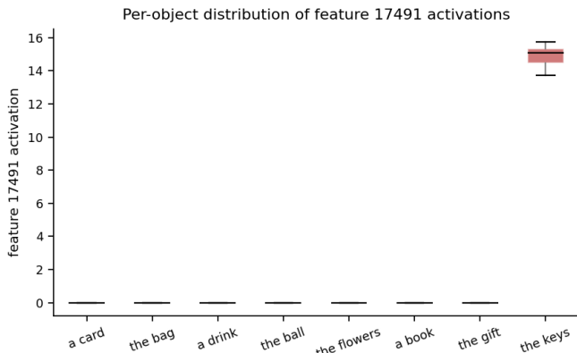
Fig. 3: Distribution of feature 17,491 activations per transferred-object choice. The “the keys” subset (red) is the clear outlier; on the other seven objects the feature is essentially silent.
