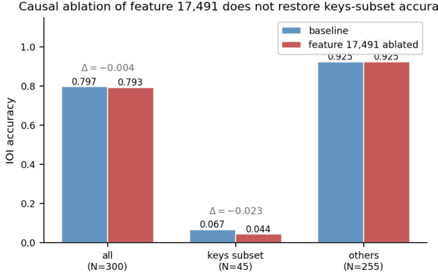
Fig. 5: Causal ablation. Zeroing feature 17,491 across all token positions of the residual stream does not restore IOI accuracy on the 45-prompt keys subset; it moves accuracy slightly in the opposite direction. This is the central negative result of the paper: the strongest statistical correlate of failure does not behave like a sufficient cause at this layer.
