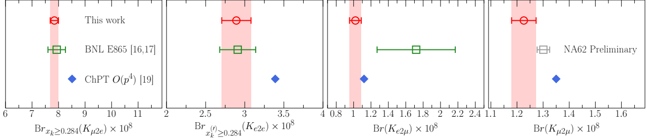
FIG. 3. Comparison of the SM predictions for the K_{\ell 2 \ell'} branching fractions with experimental measurements from BNL E865 and the preliminary NA62 result. The ChPT predictions at O(p^4) from Ref. [19] are also shown.
