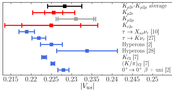
FIG. 5. |V_{us}| values obtained in this work (excluding the noisy K_{e2\mu} result), together with existing determinations. Inner error bars denote theory uncertainties.
