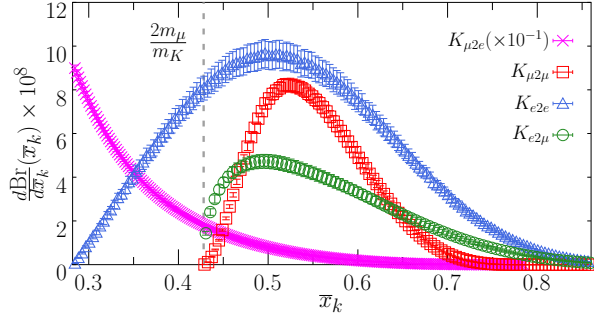
FIG. 4. Differential branching fractions for K_{\ell 2 \ell'} as defined in Eq. (12). The data corresponding to K_{\mu 2e} have been divided by 10 for better visualization.
