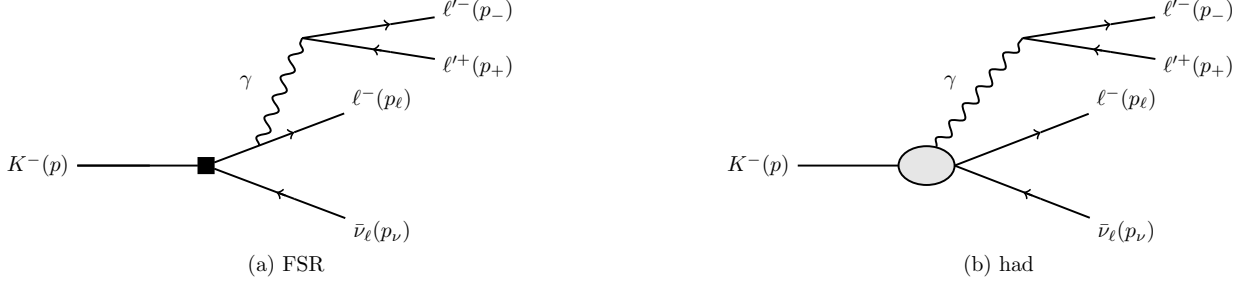
FIG. 1. Leading-order diagrams contributing to K^- \rightarrow \ell^- \bar{\nu}_\ell \ell'^+ \ell'^- : (a) final-state radiation from the charged lepton line; (b) emission of the virtual photon from the kaon. For \ell = \ell' the exchange contribution must be included (see Eq. 8). The black box in the left panel corresponds to the insertion of the four-fermion weak operator of the Fermi effective theory.
