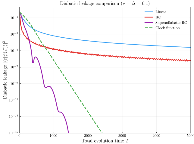
FIG. 2. Numerical computation of the diabatic leakage via exact diagonalization of the two-level Hamiltonian (8). Four different schedules are considered: linear, Roland–Cerf, superadiabatic Roland–Cerf, and the DC clock function, which can be interpreted as the linear schedule reparametrized by the DC clock. While the linear and Roland–Cerf schedules yield a power-law decay, the reparametrized schedules suppress diabatic transitions near-exponentially. Both RC-type schedules display Stückelberg oscillations arising from coherent interference between nonadiabatic transitions.
