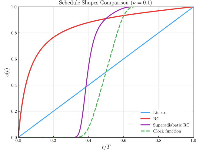
FIG. 1. A visualization of three different schedule profiles: (a) The linear ramp profile s(t) = t/T . (b) The Roland-Cerf schedule (10) mirroring the behavior of the spectral gap. (c) The Roland-Cerf schedule reparametrized by a DC clock, which we call superadiabatic RC. Also shown is the behavior of the DC clock function, whose endpoint derivatives vanish and which thereby near-exponentially suppresses diabatic transitions.
