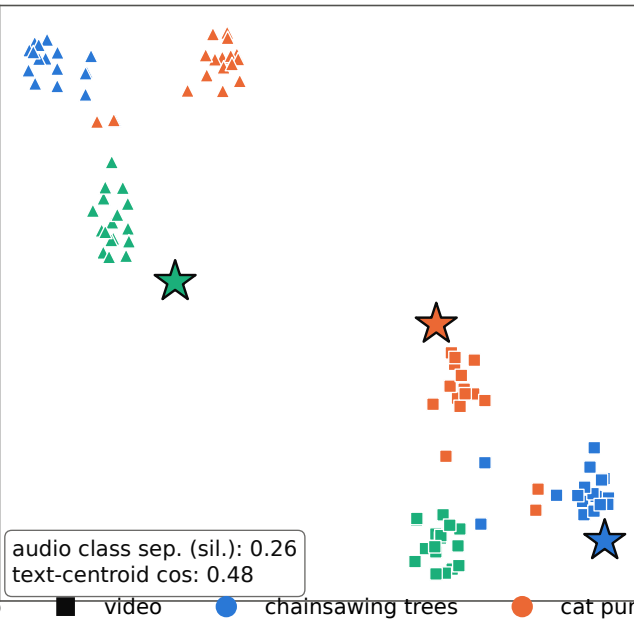
GRAM (1.4B full-FT)
