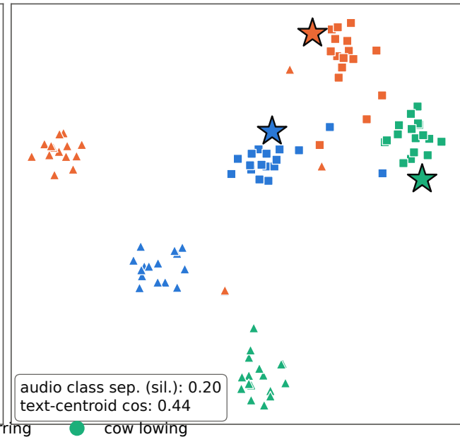
SCA (4.8M LoRA, ours)
