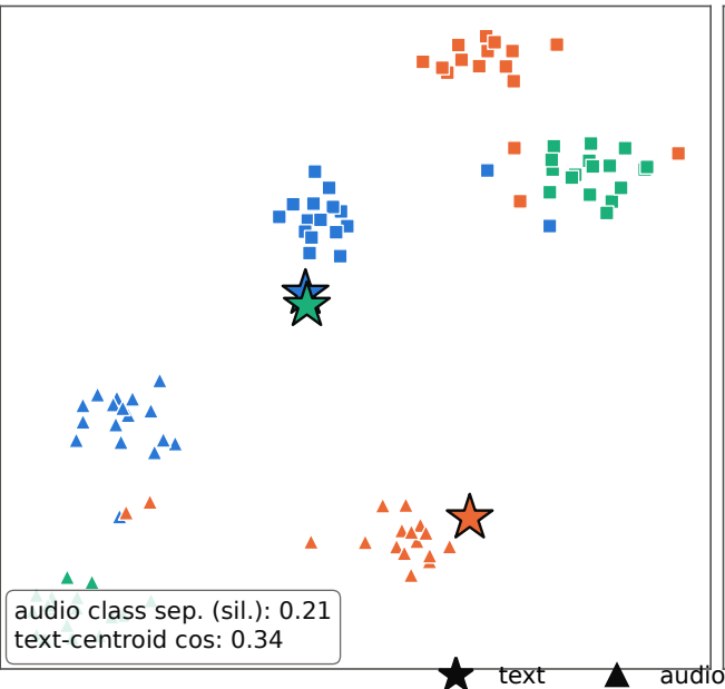
VAST (shared init.)
