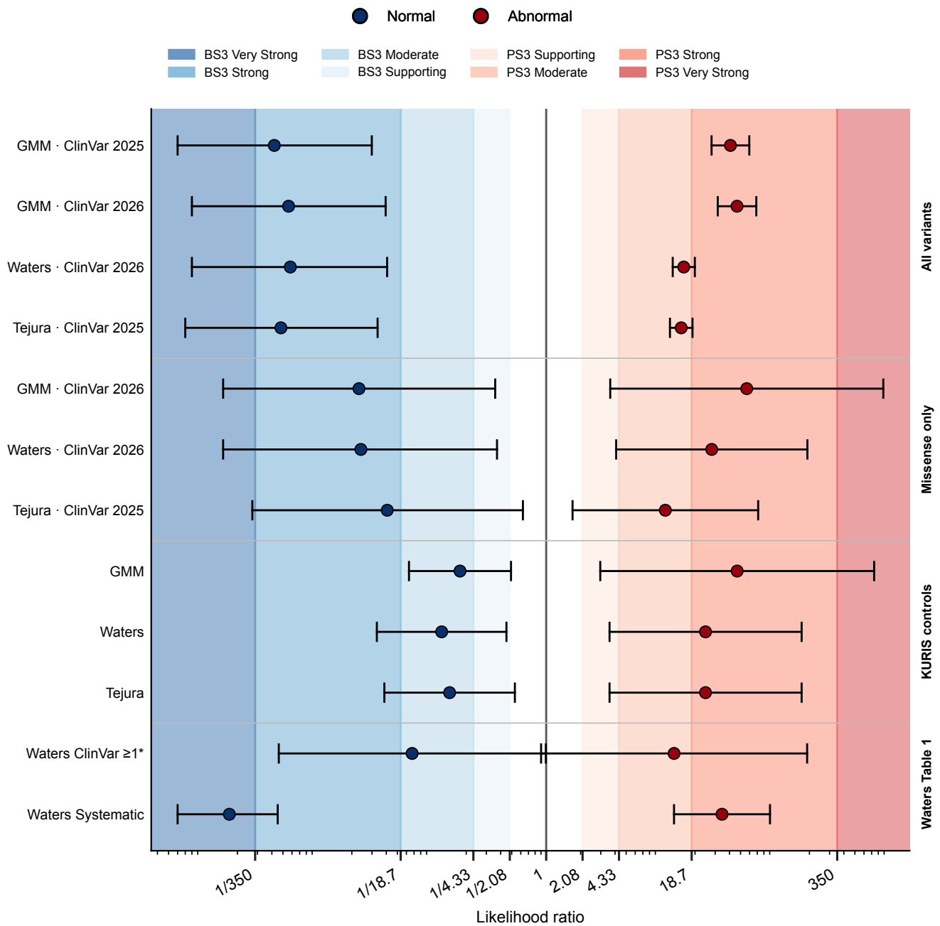
Supplementary Figure 3. Likelihood ratios across functional-classification methods and control sets.
