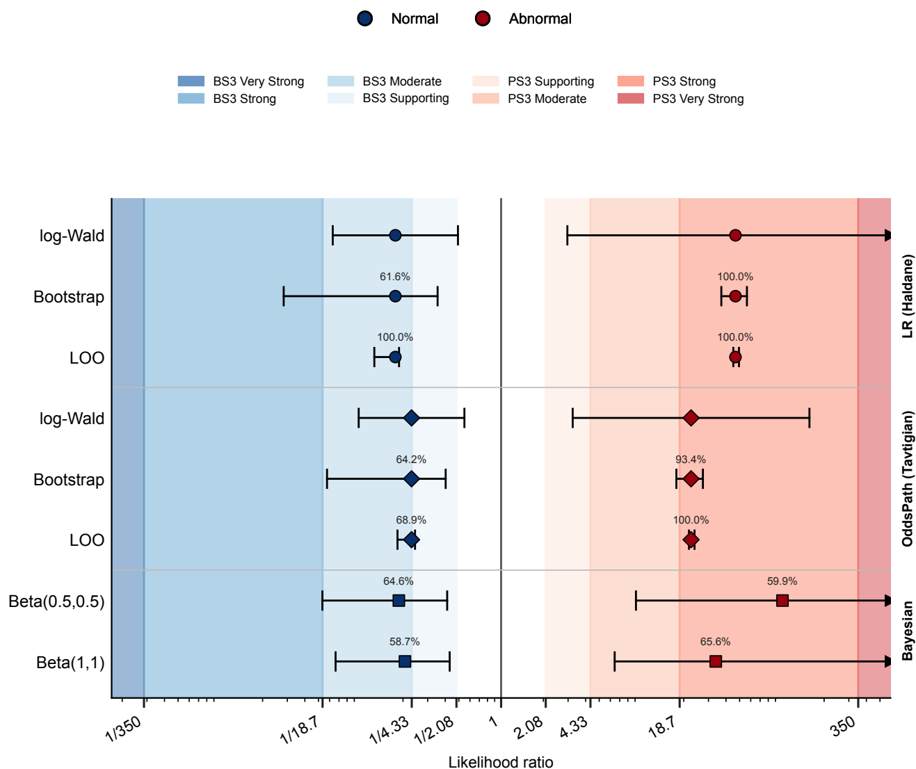
Supplementary Figure 4. Stability of the KURIS/NDD missense likelihood-ratio estimate across estimators.
