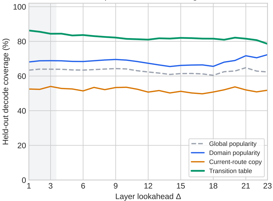
Expert-selection coverage
