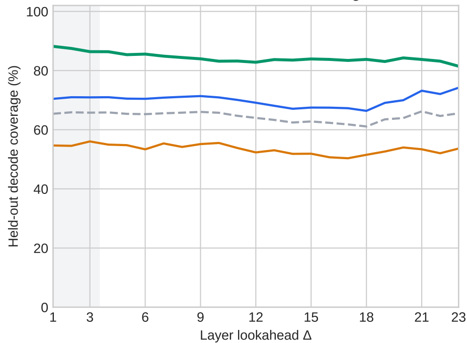
Selected routed-mass coverage
