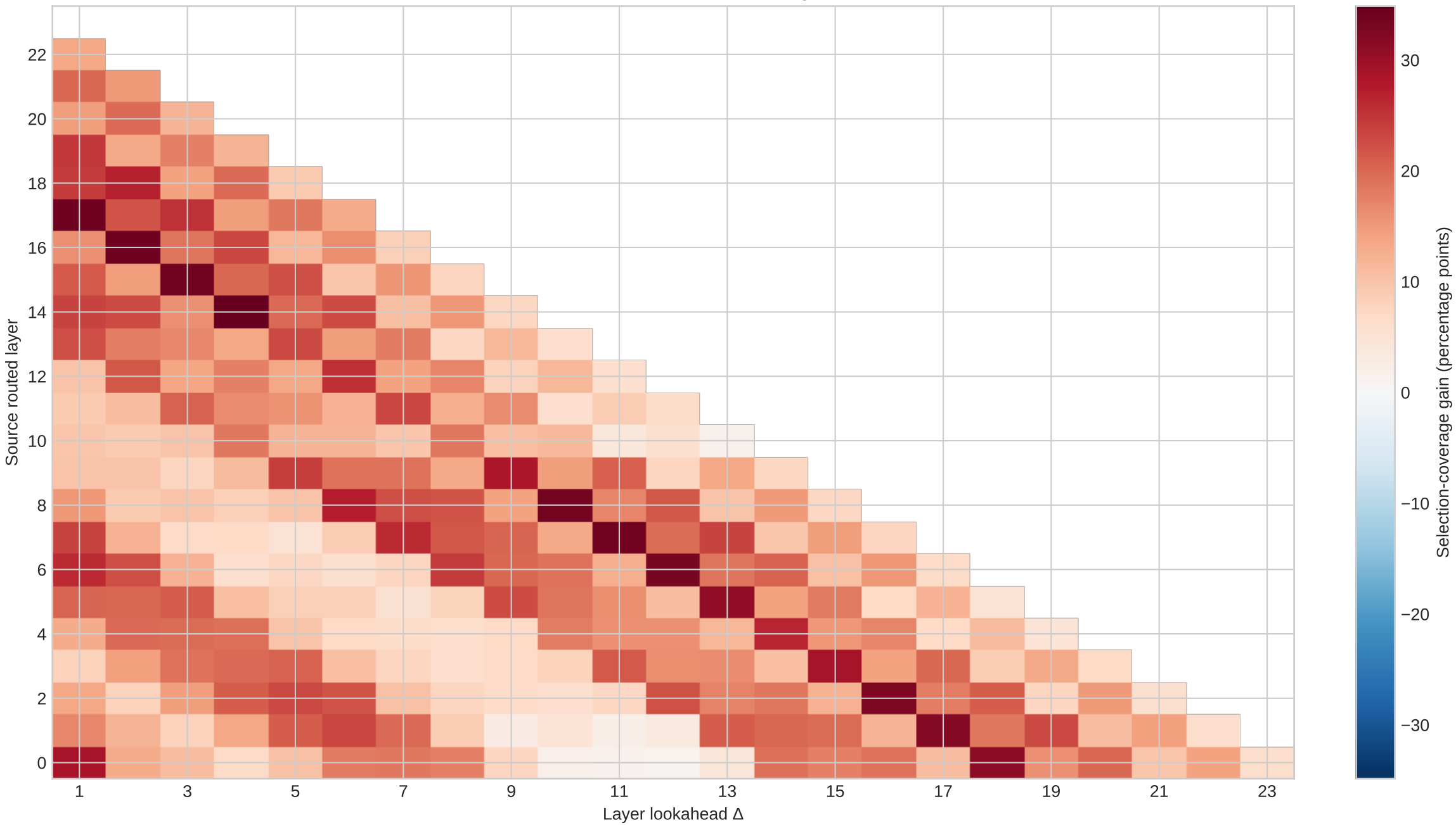
Transition gain over the stronger cheap baseline Held-out decode selection coverage, K=8
