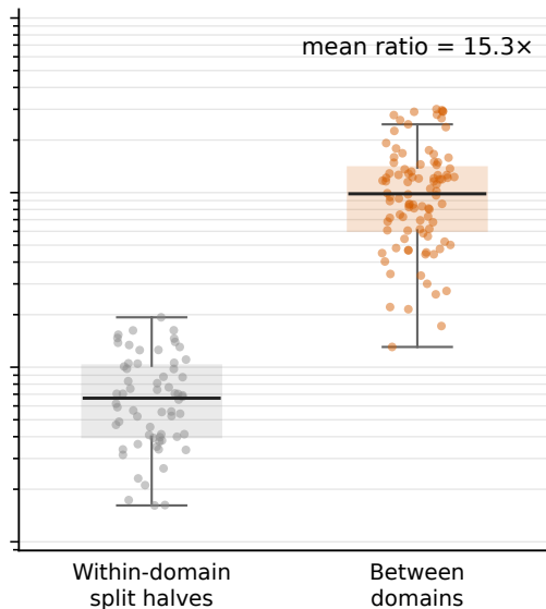
(b) Decode
