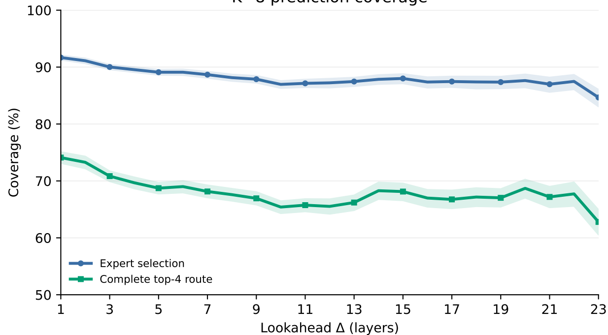
K=8 prediction coverage
