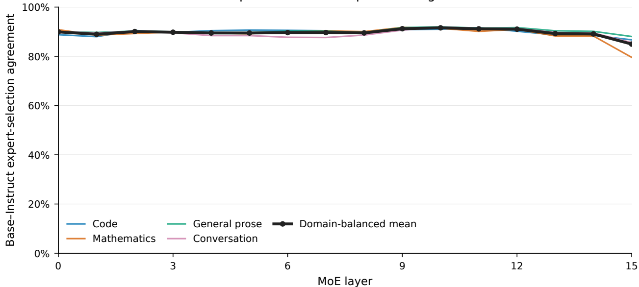
How much of each token's top-8 route survives post-training
