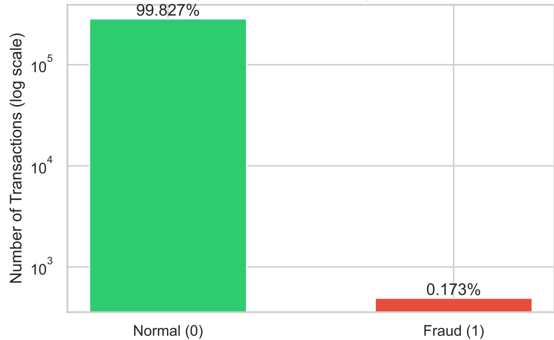
Class Distribution - Log Scale
