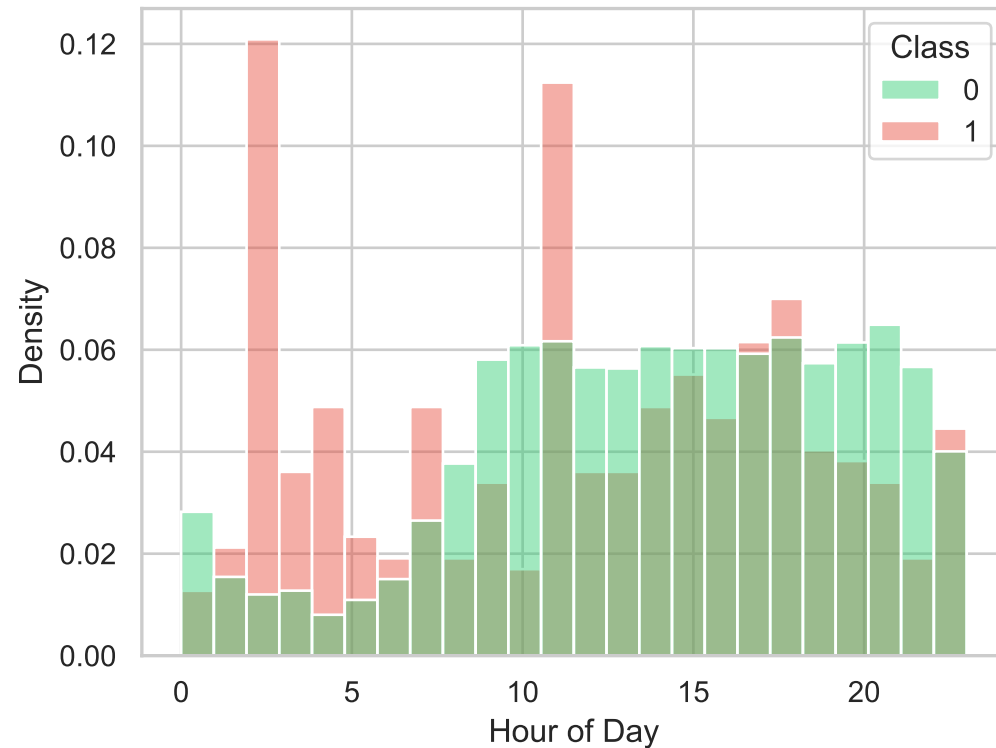
Transaction Time of Day by Class
