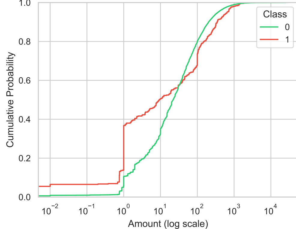
Cumulative Amount Distribution
