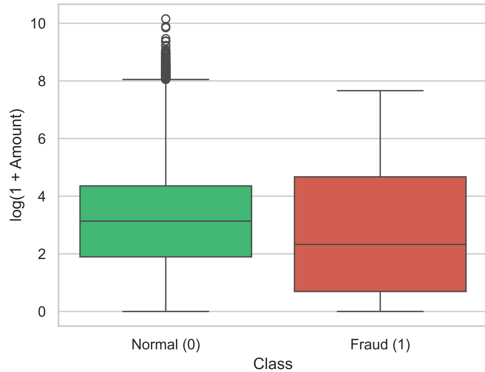
Transaction Amount by Class
