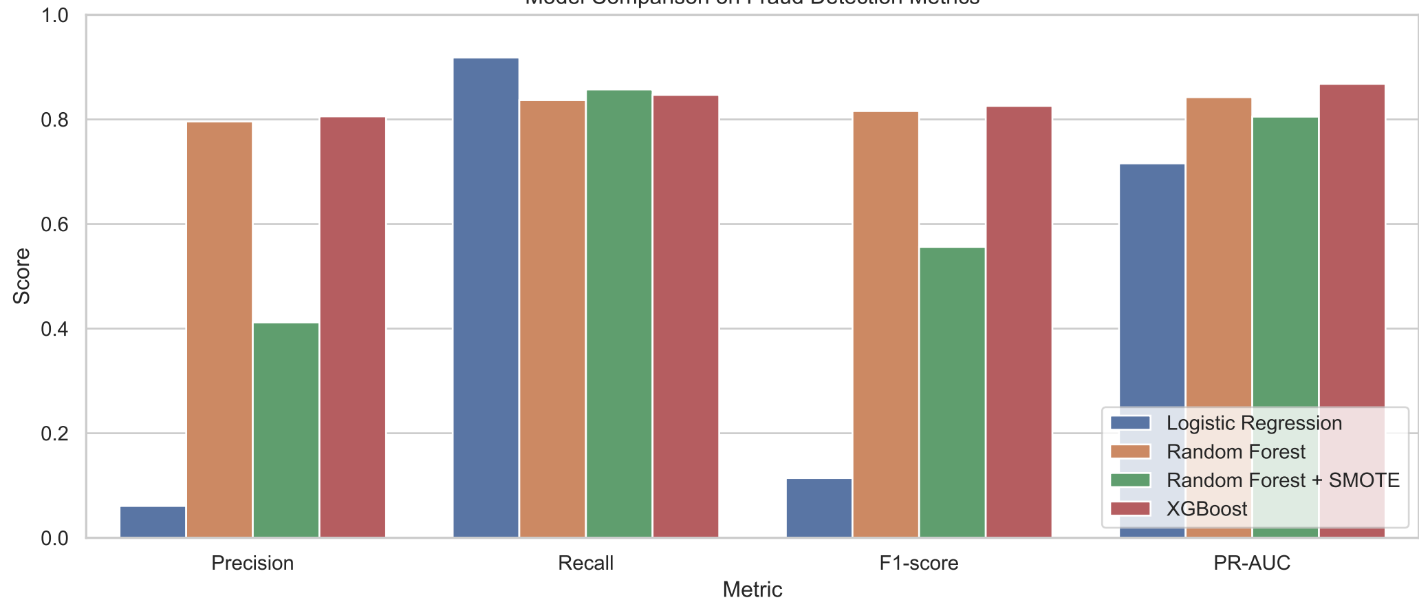
Model Comparison on Fraud Detection Metrics
