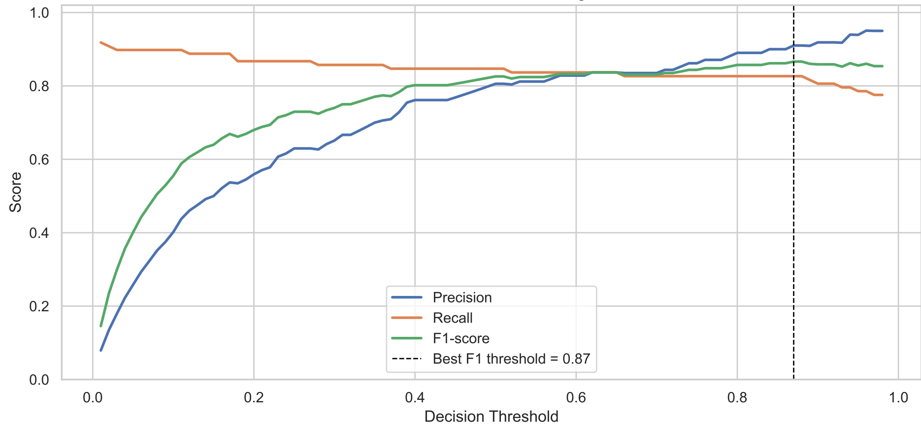
XGBoost Threshold Tuning
