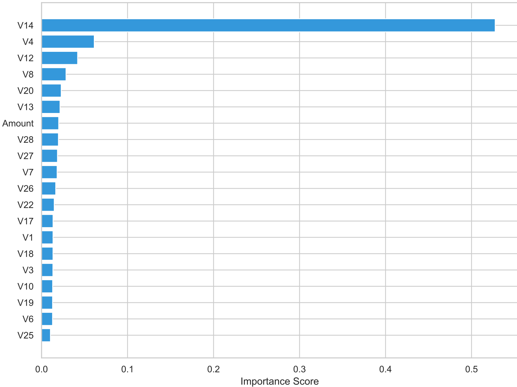
Top 20 Feature Importance - XGBoost
