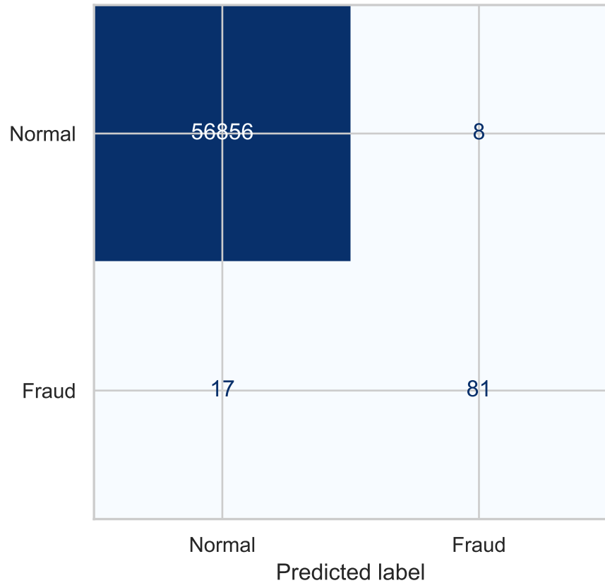
XGBoost Confusion Matrix Threshold = 0.87
