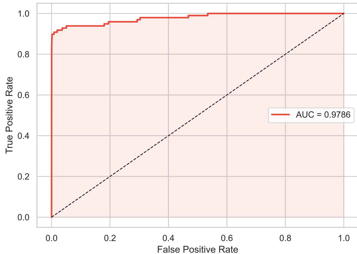
ROC Curve
