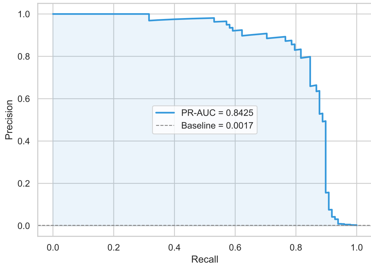
Precision-Recall Curve
