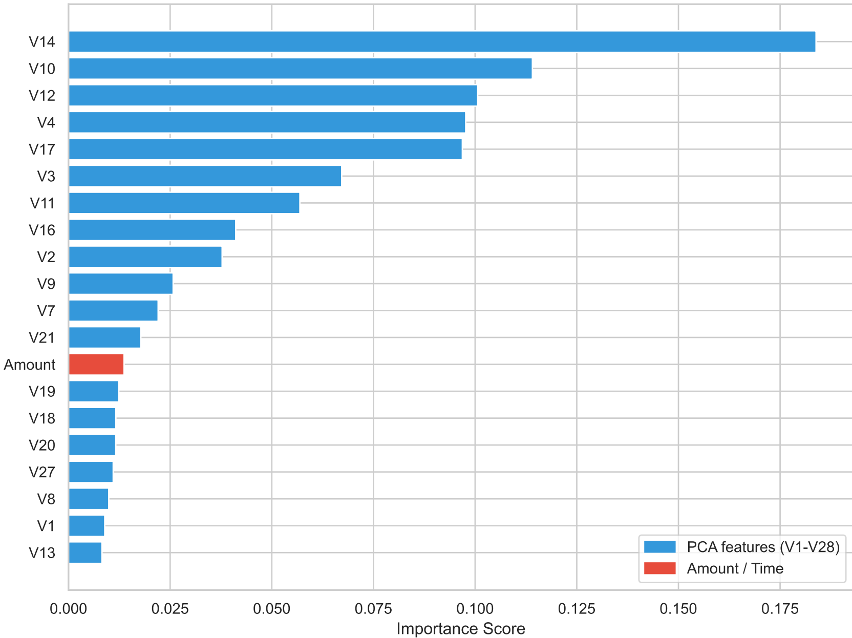
Top 20 Feature Importance - Random Forest
