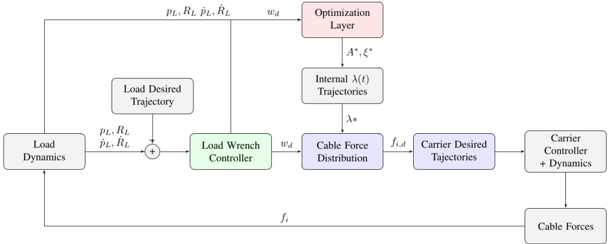
Figure 3.2: Overall classical control pipeline scheme, including the load-wrench controller (green block), the carrier-trajectory generator (blue blocks), and the optimization layer (red block).
