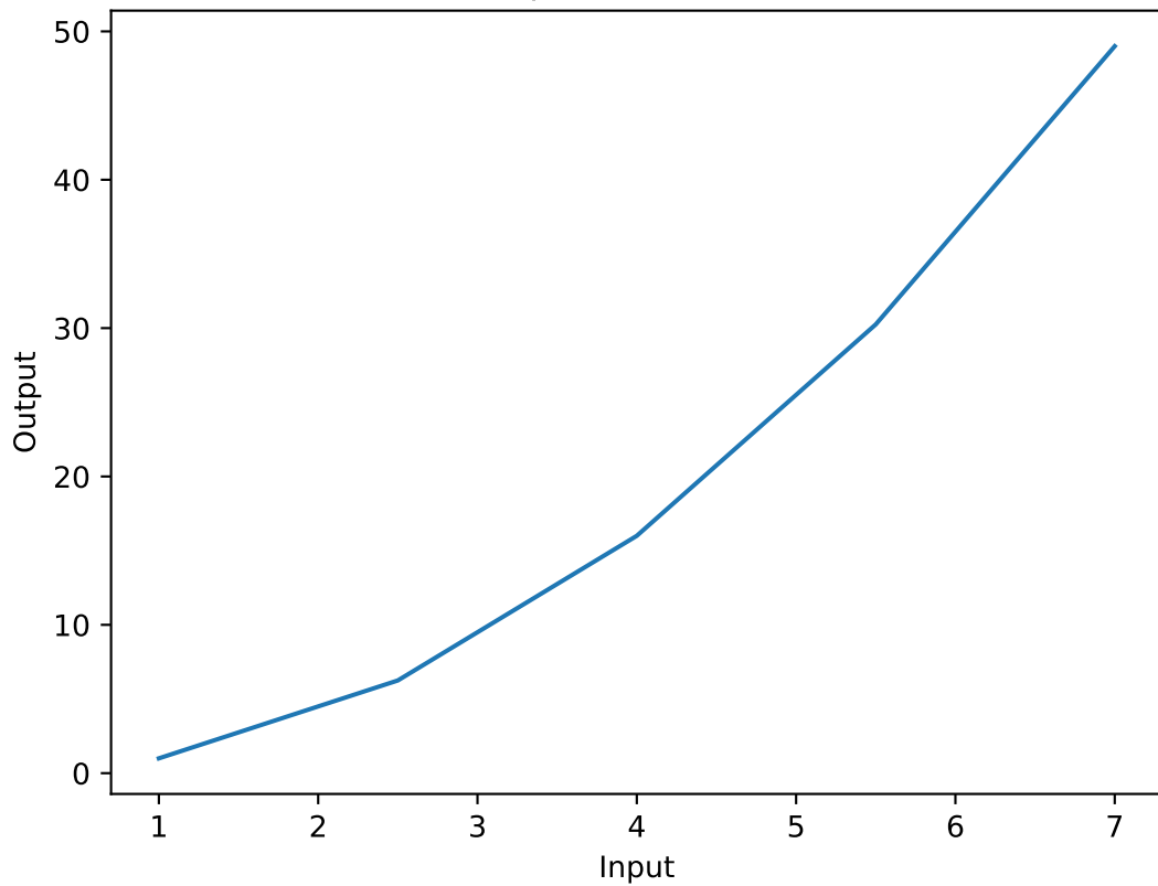
Square Function
