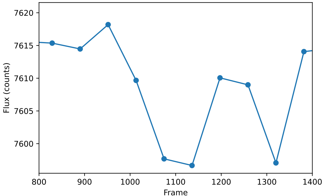
Binned transit light curve (good frames only)
