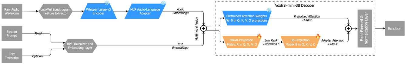
Figure 1: Overview of the multimodal Voxtral-mini-3B fine-tuning pipeline. Fused embeddings flow through parallel pretrained weights and trainable low-rank matrices A and B across the Q, K, V, O projections. The combined attention representations are summed and passed through the frozen Feed-Forward and Normalization layers to generate one label from the four-class emotion set. Blue modules denote frozen pretrained components, whereas orange modules represent trainable parameters.
