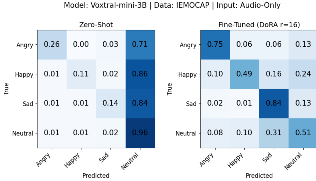
Figure 2: Normalized confusion matrices on IEMOCAP for Voxtral-mini-3B, comparing zero-shot inference and PEFT fine-tuning (DoRA r=16 ). Fine-tuning reduces the strong Neutral-class collapse and improves class-wise separation.
