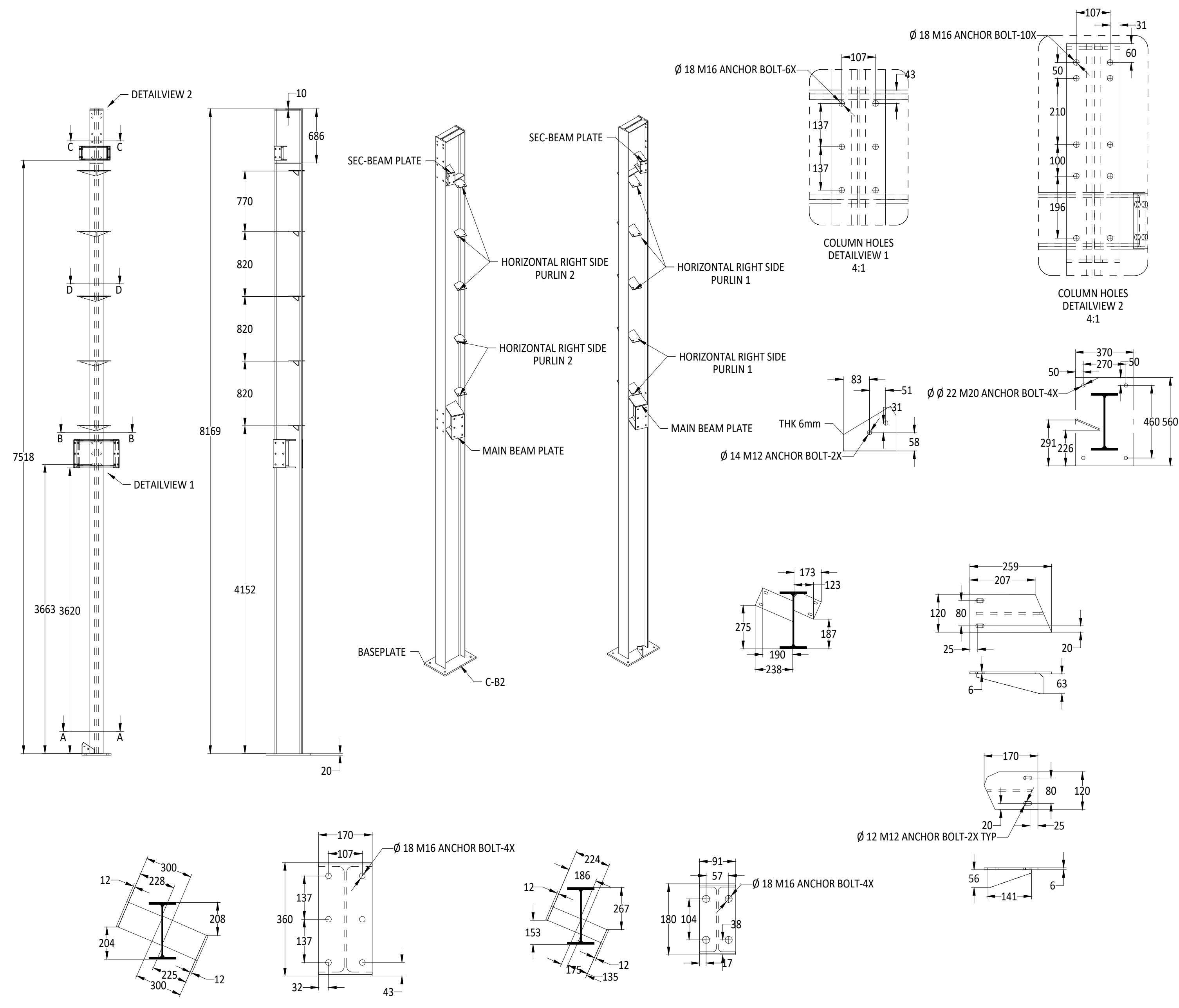
COLUMN C-B2 FABRICATION DETAILS
