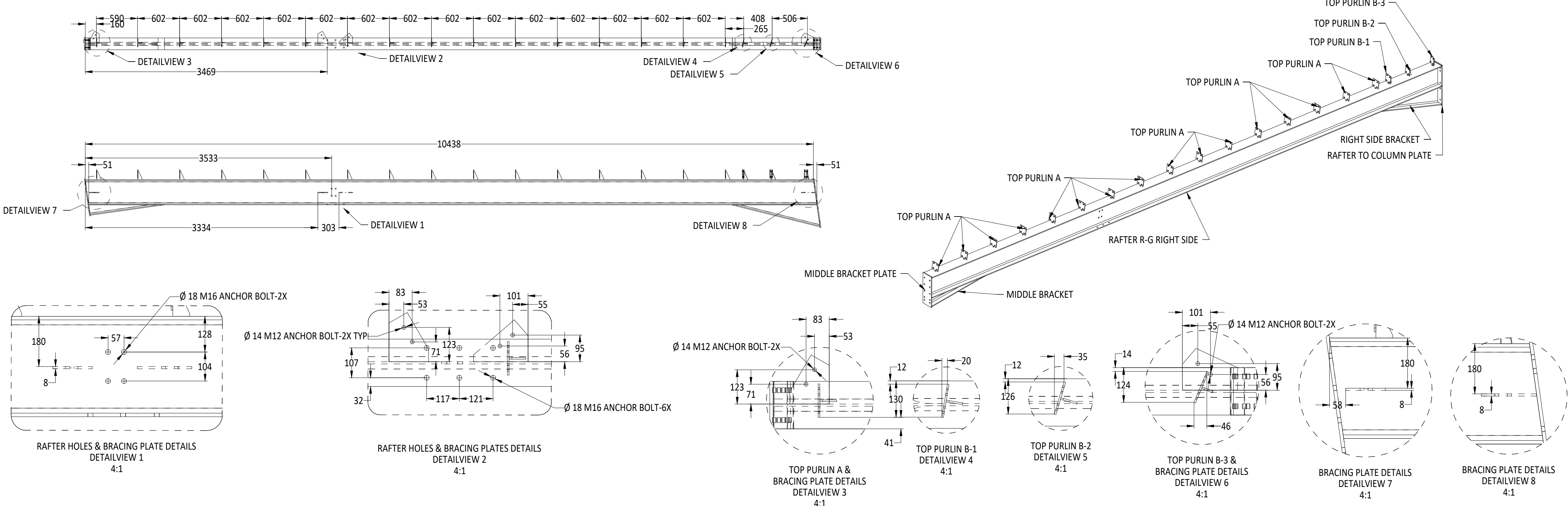
RAFTER R-G RIGHT FABRICATION DETAILS
