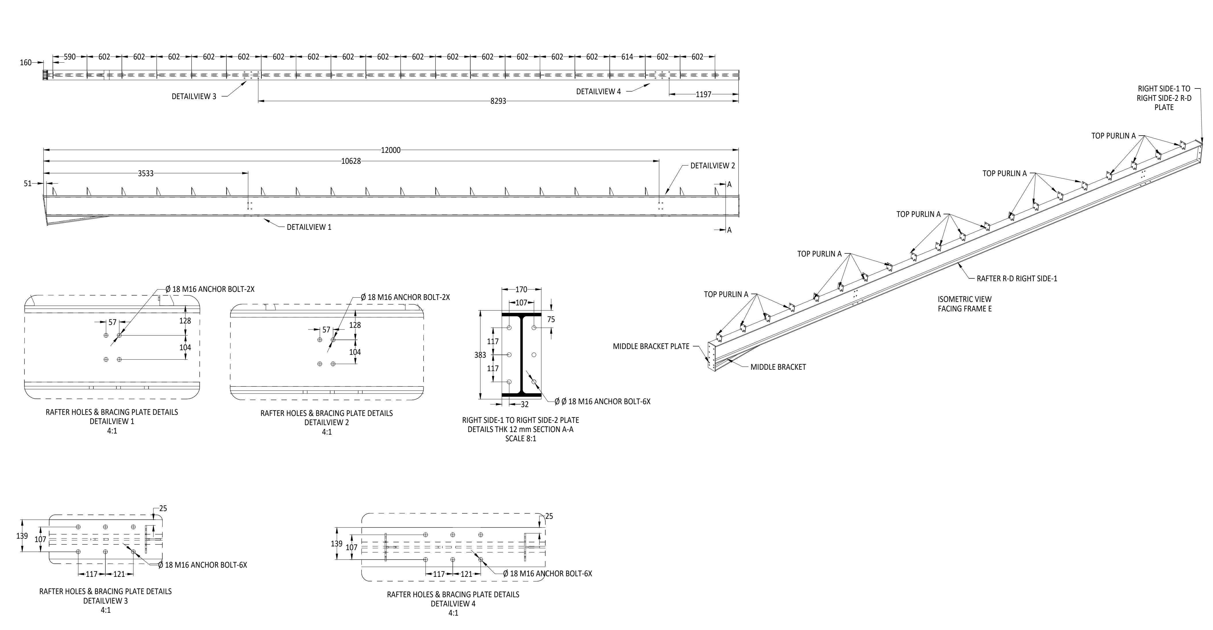
RAFTER R-D RIGHT SIDE-1 FABRICATION DETAILS
