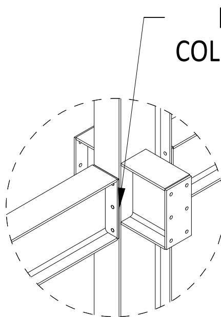
DETAILVIEW 3 4:1
