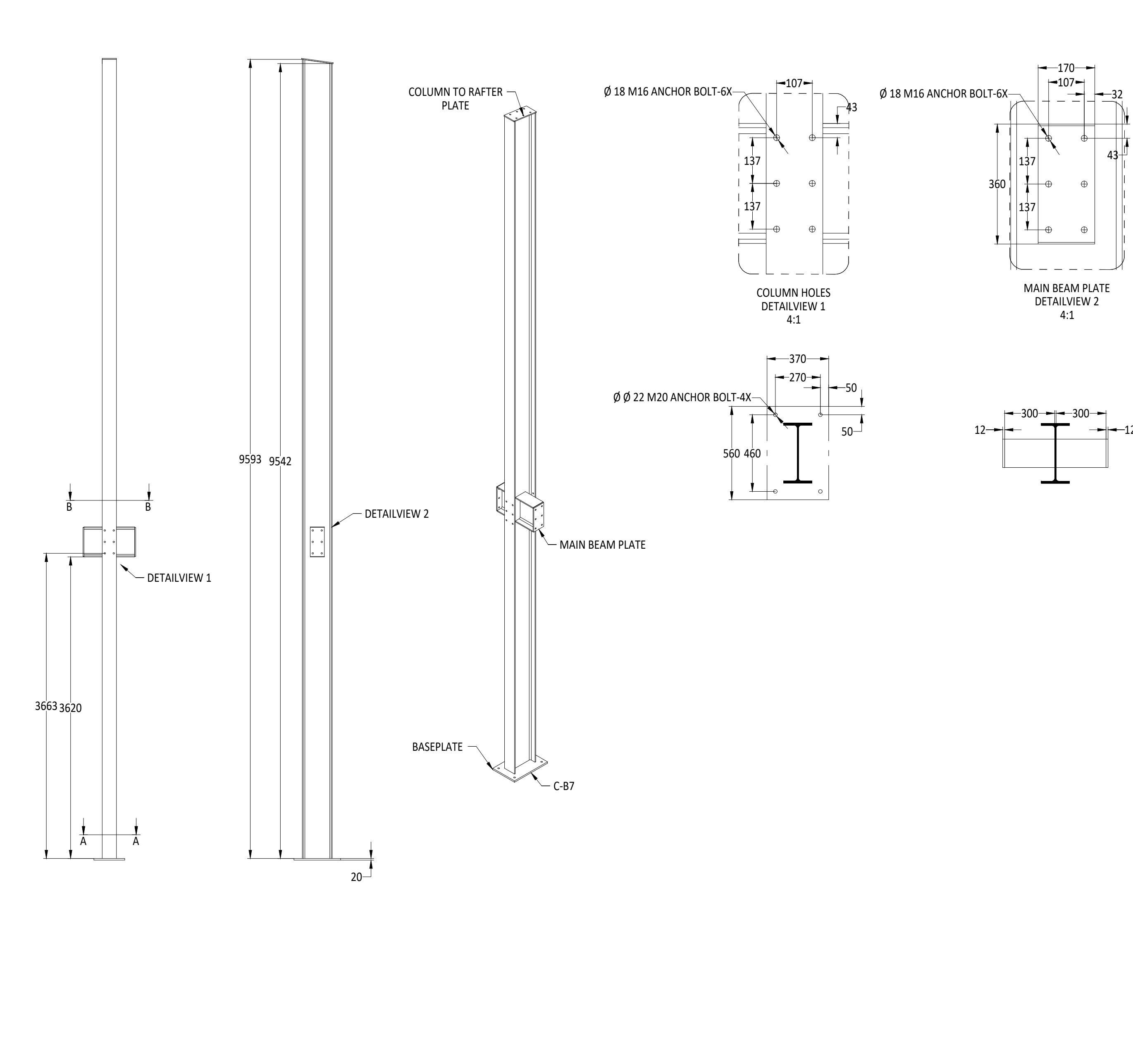
COLUMN C-B7 FABRICATION DETAILS
