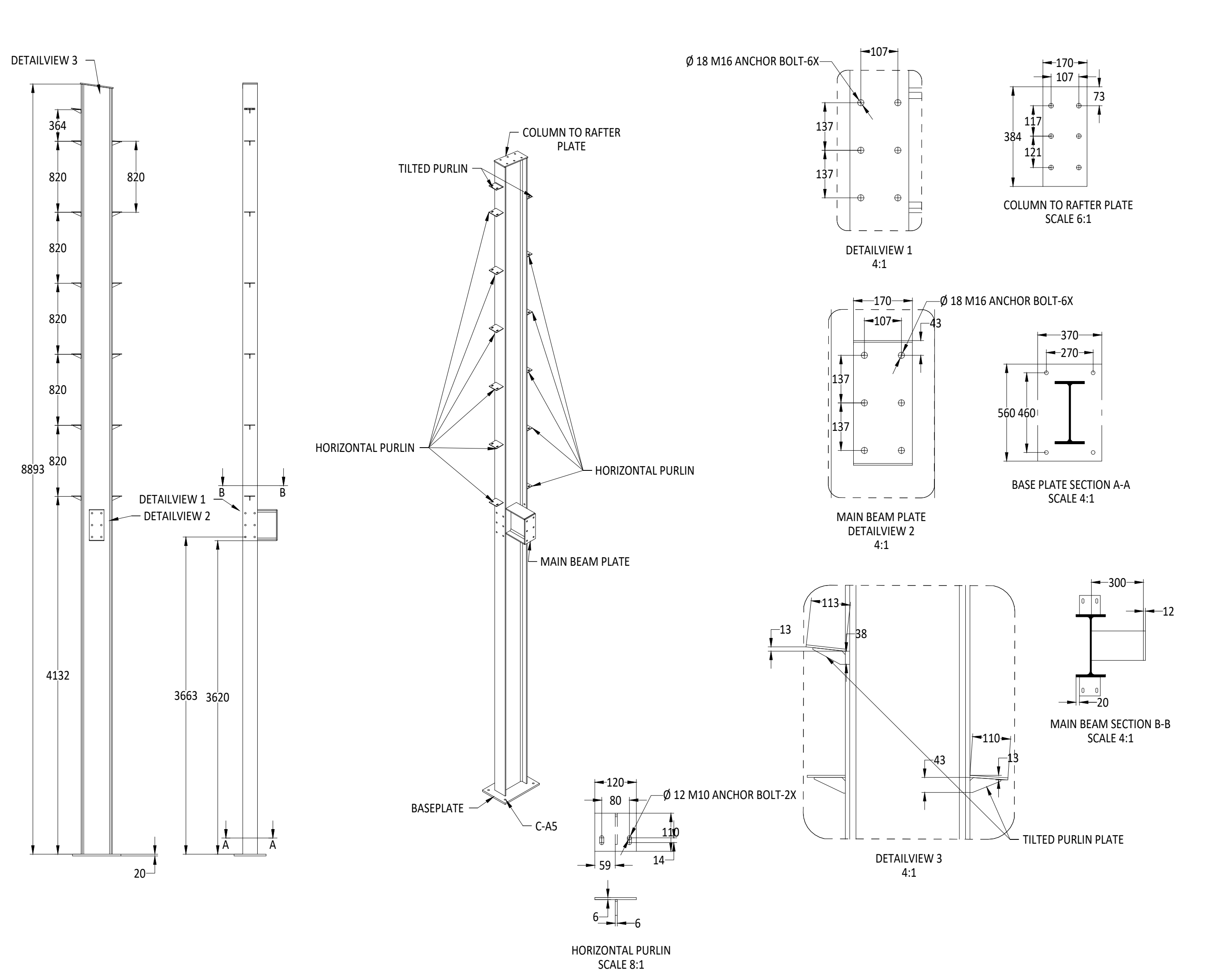
COLUMN C-A5 FABRICATION DETAILS
