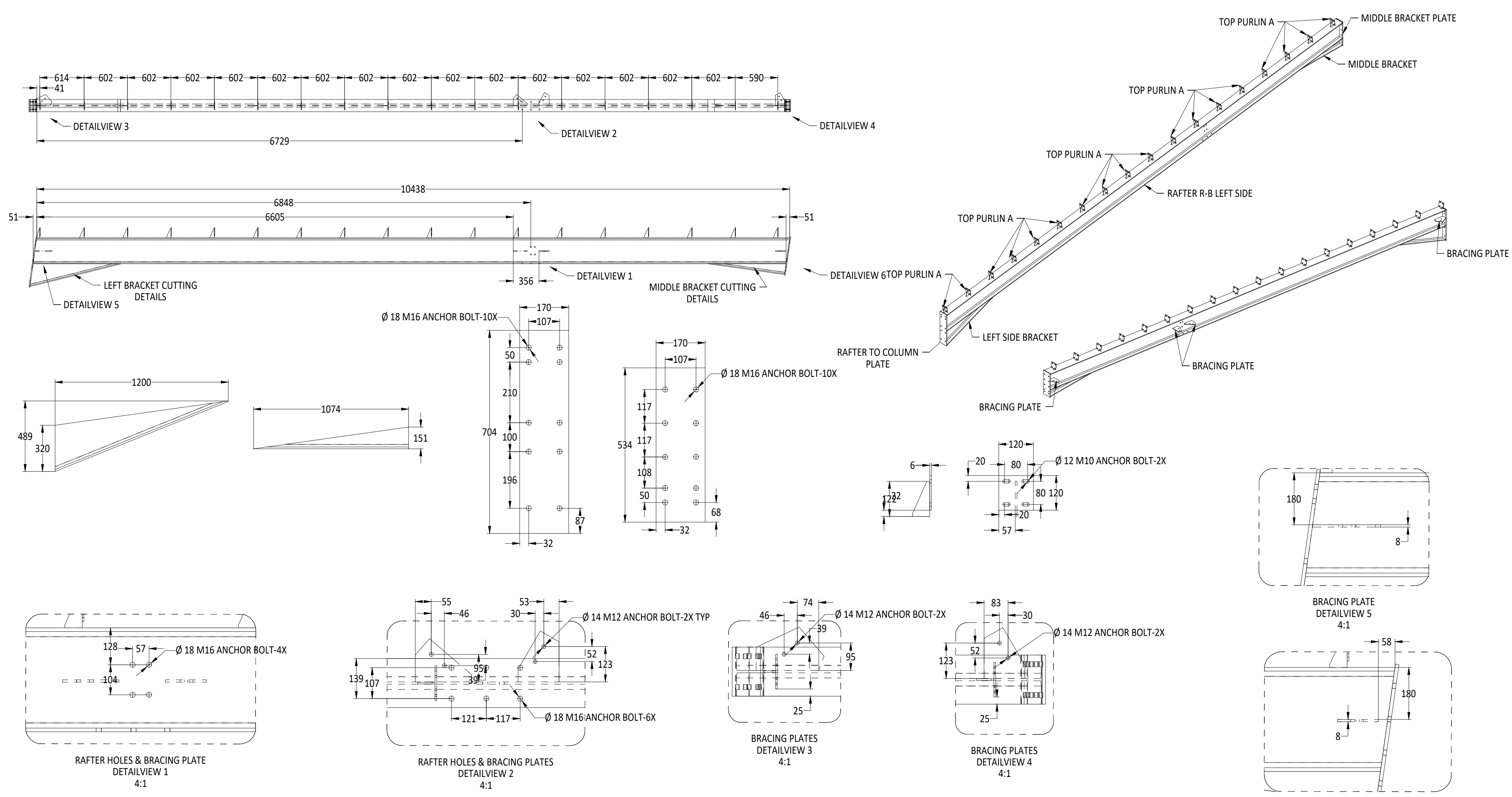
RAFTER R-B LEFT SIDE FABRICATION DETAILS
