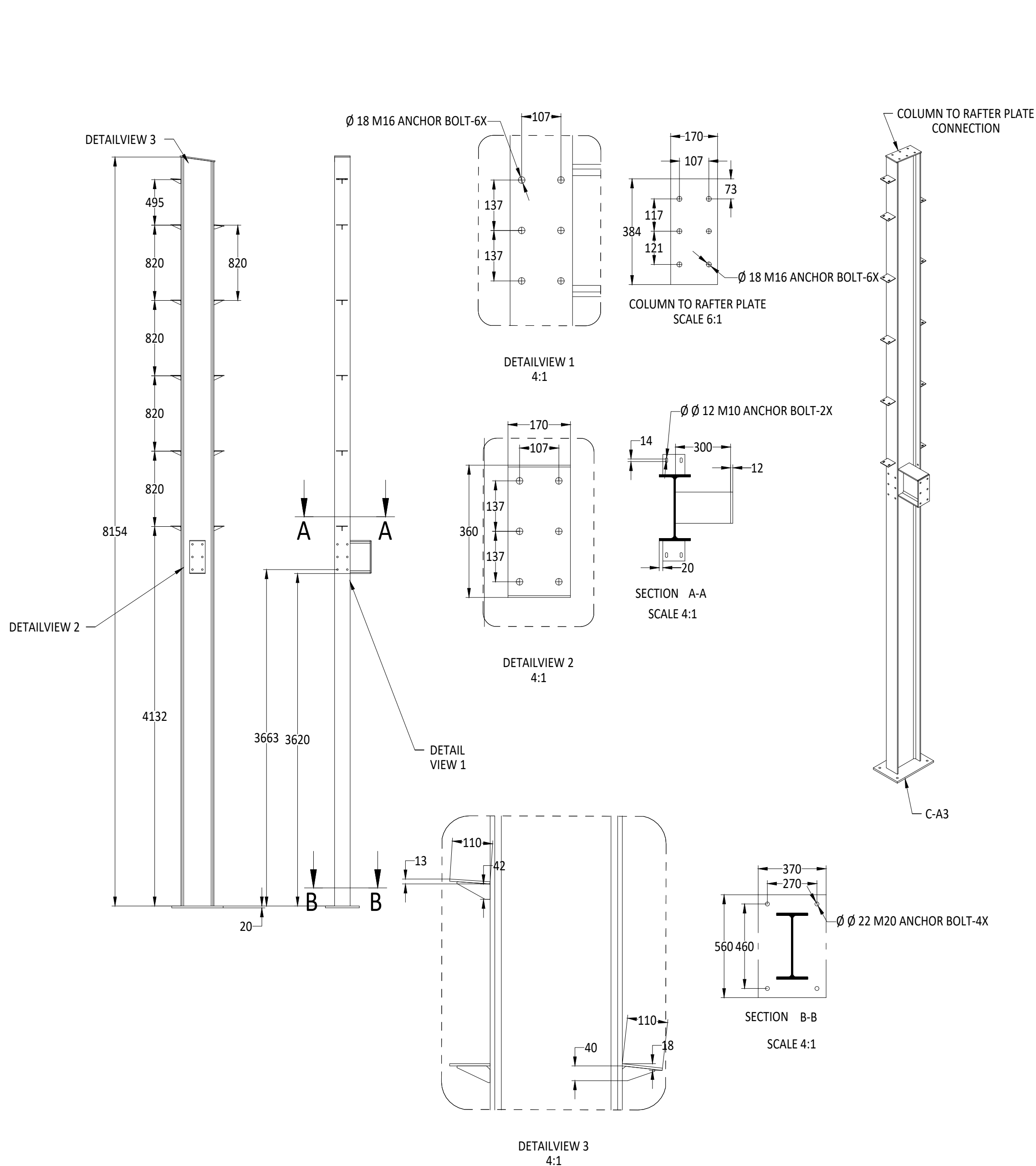
COLUMN C-A3 FABRICATION DETAILS
