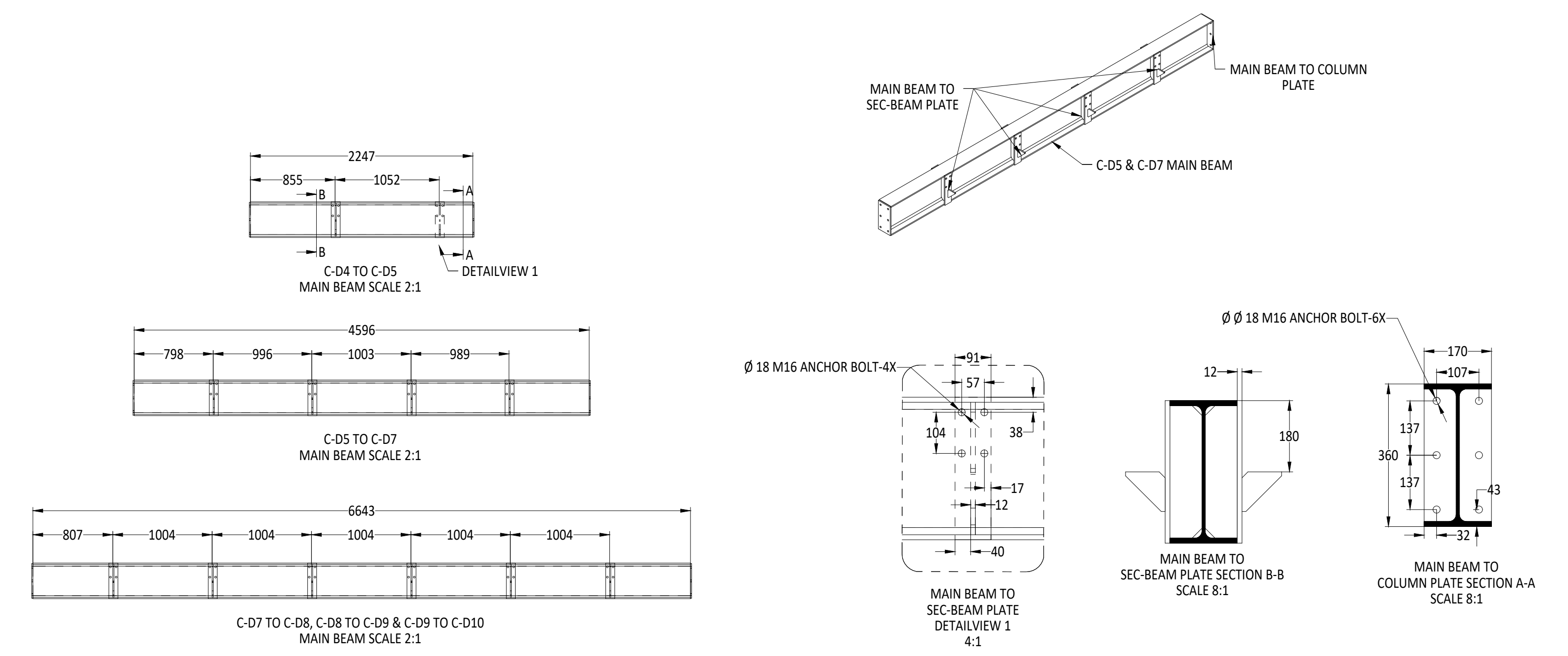
MAIN BEAMS FABRICATION DETAILS
