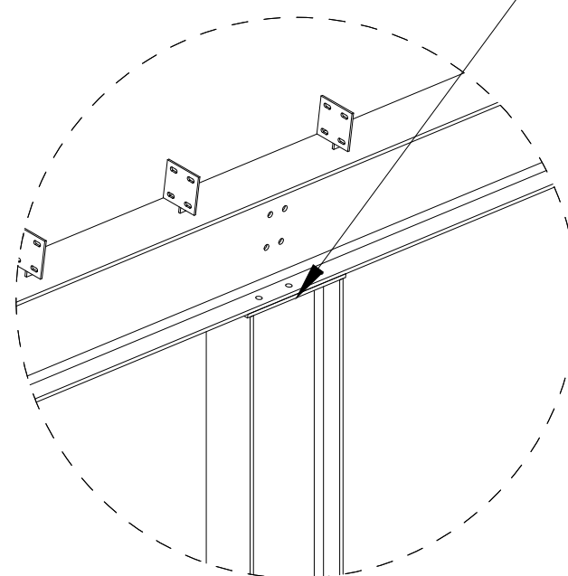
DETAILVIEW 4 4:1
