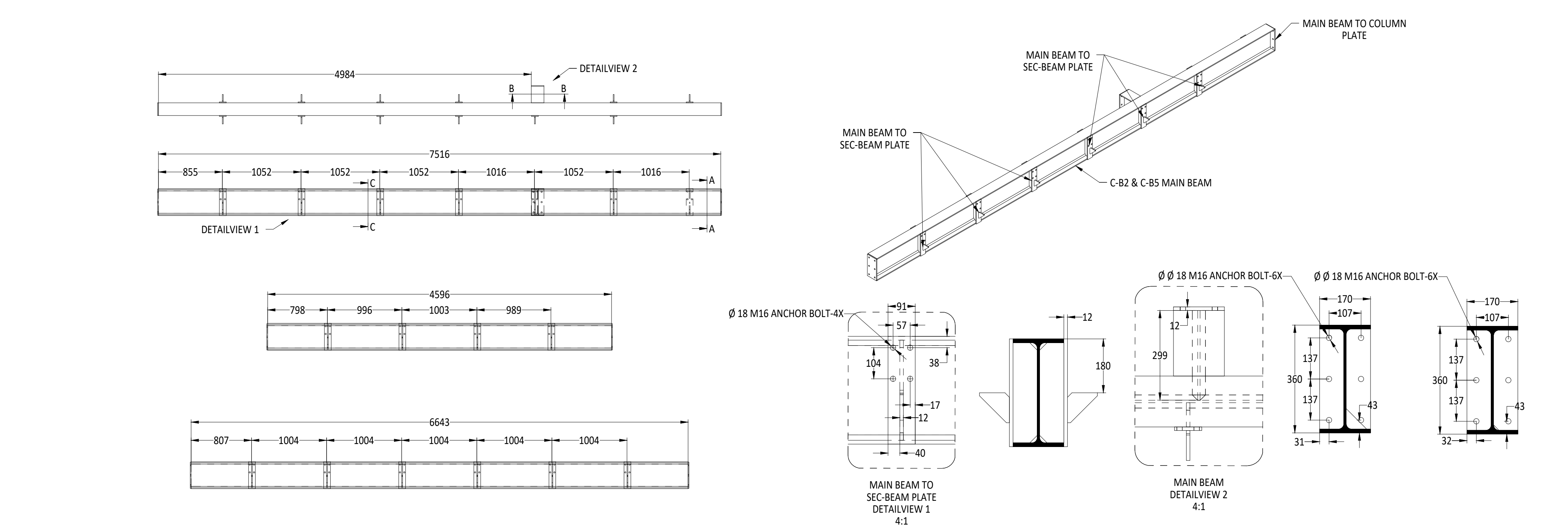
RAFTER R-B RIGHT SIDE-2 FABRICATION DETAILS
