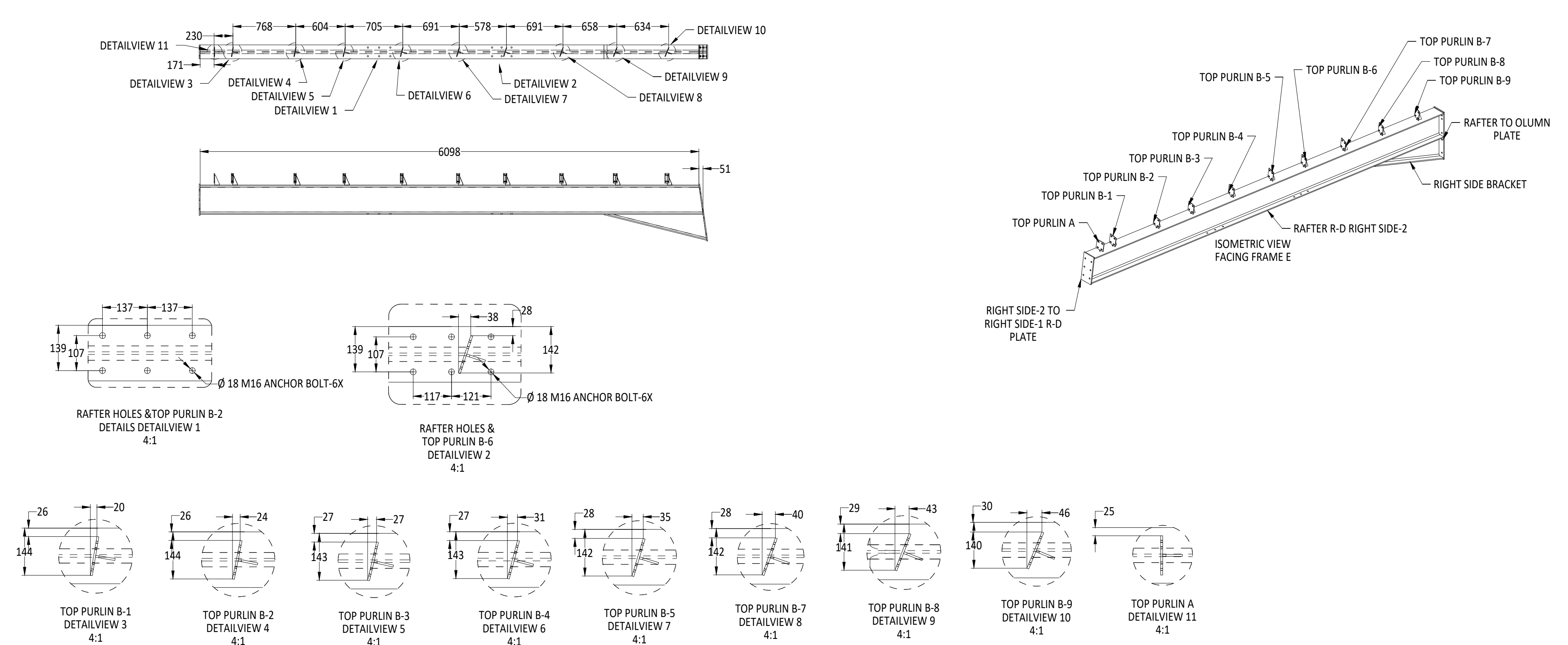
RAFTER R-D RIGHT SIDE-2 FABRICATION DETAILS
