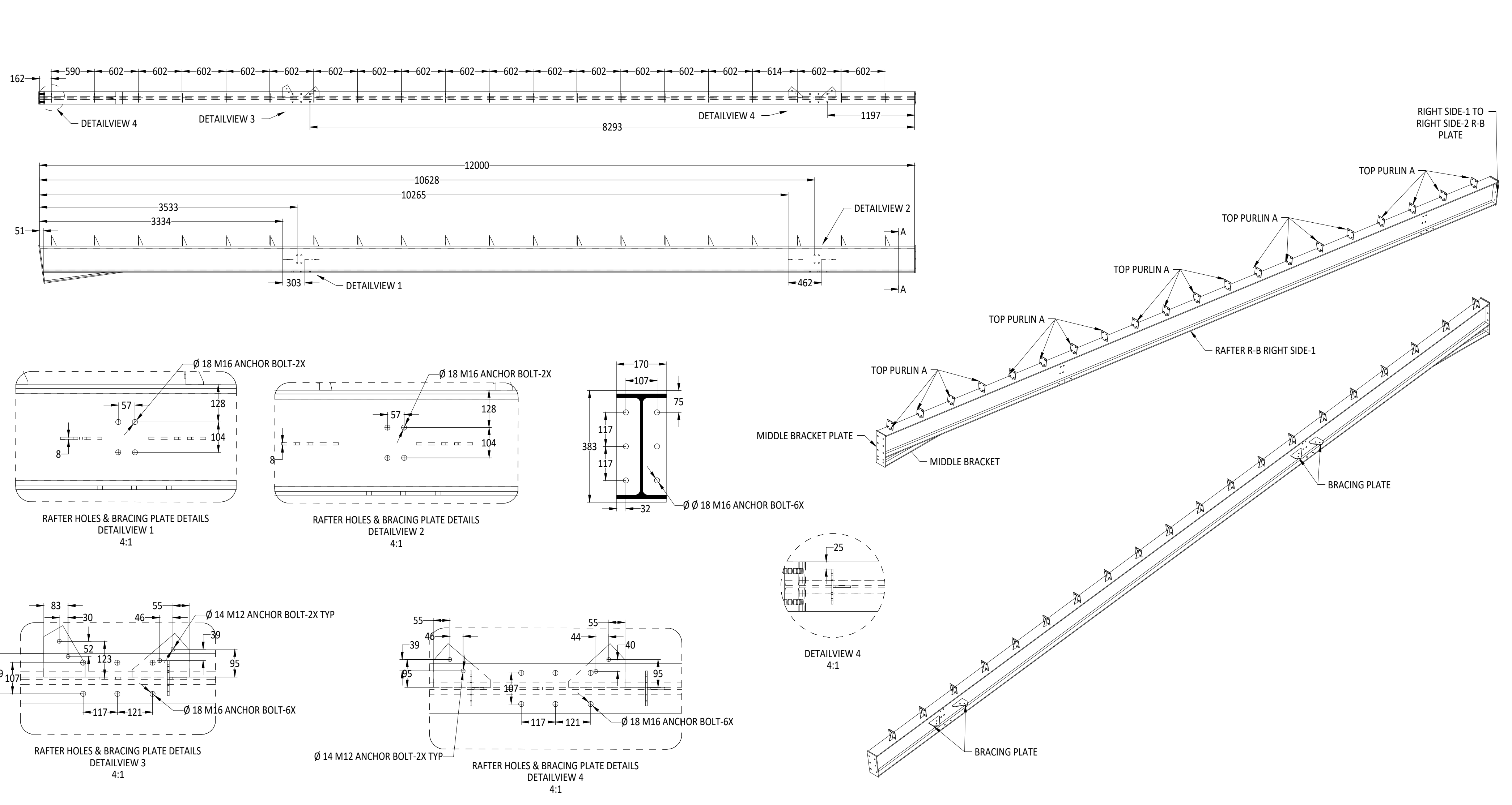
RAFTER R-B RIGHT SIDE-1 FABRICATION DETAILS
