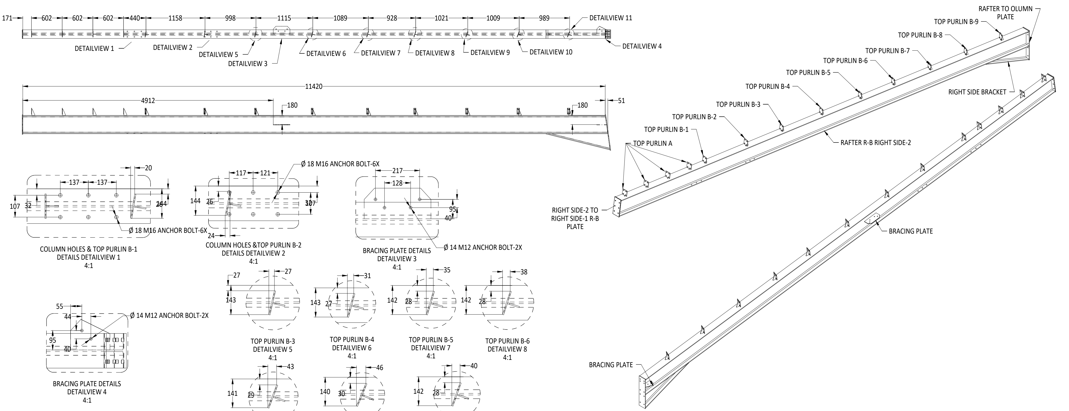
RAFTER R-B RIGHT SIDE-2 FABRICATION DETAILS
