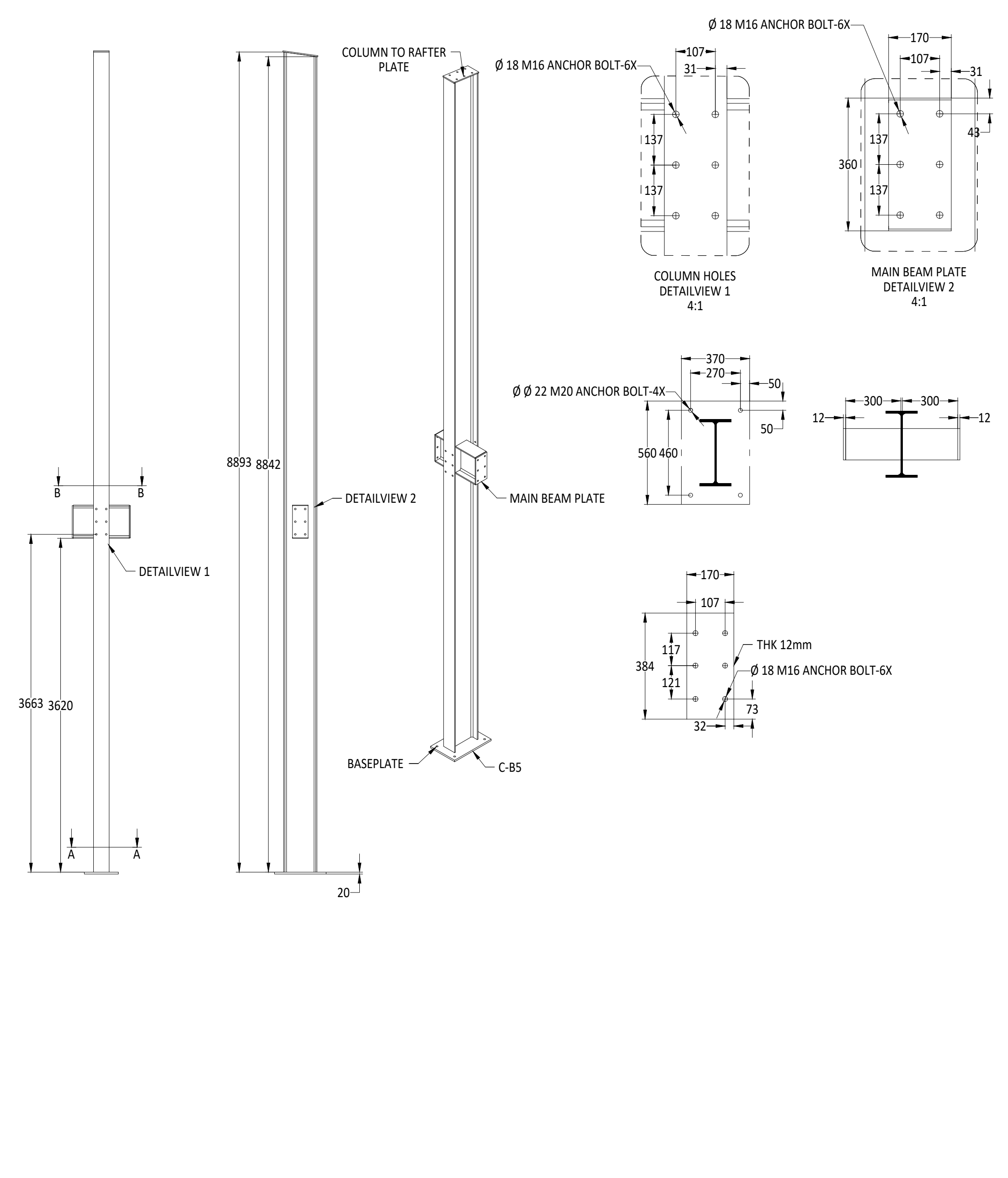
COLUMN C-B5 FABRICATION DETAILS
