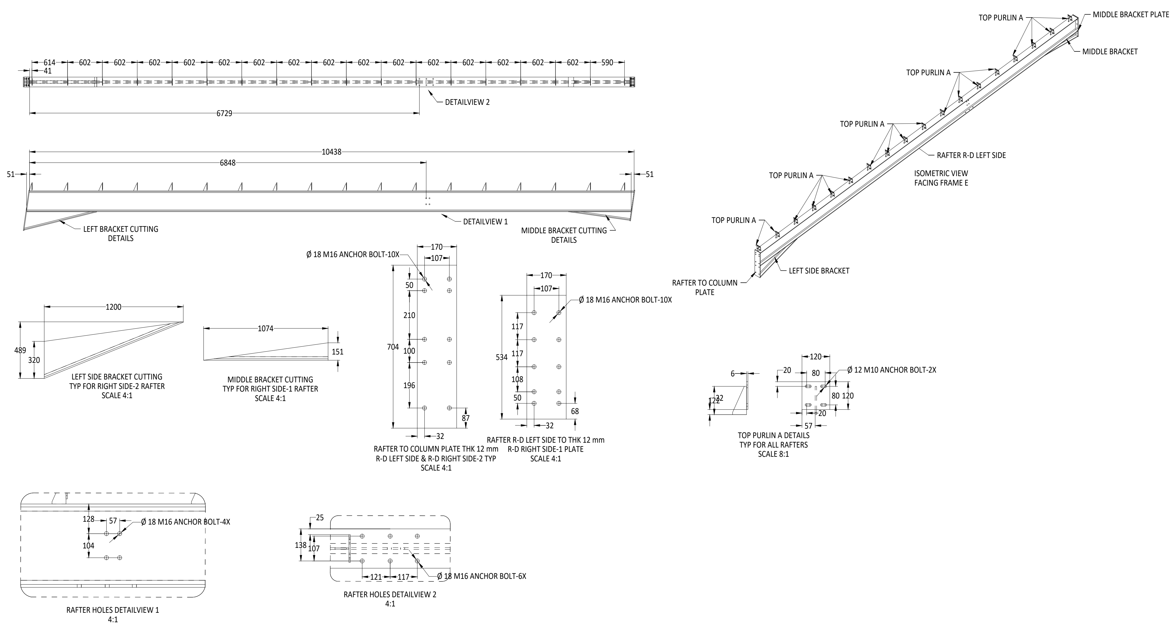
RAFTER R-D LEFT SIDE FABRICATION DETAILS
