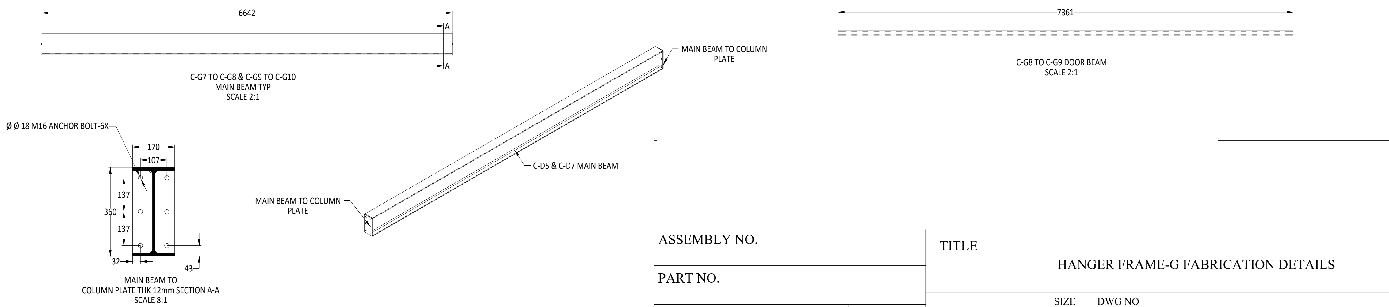
MAIN BEAMS FABRICATION DETAILS
