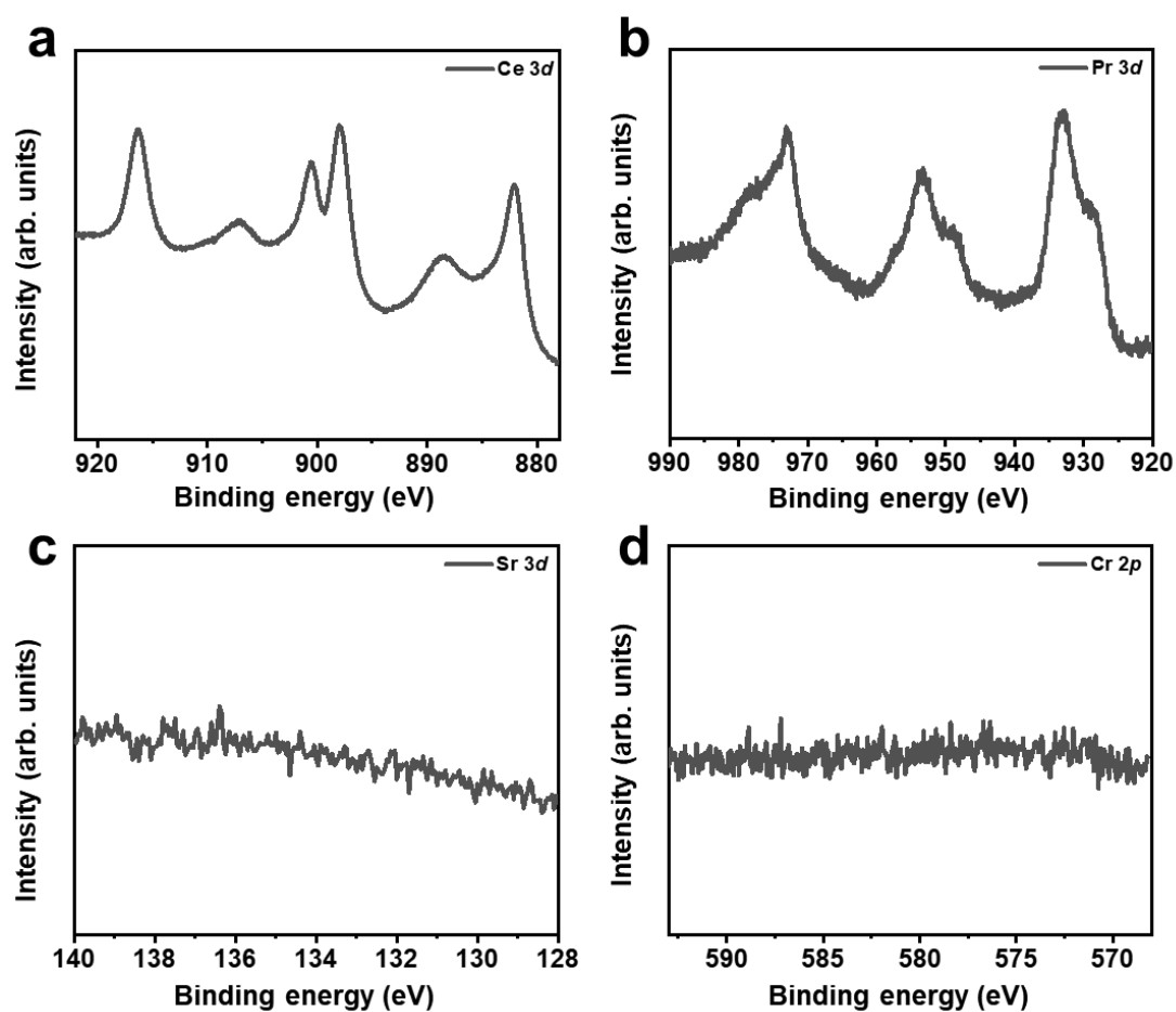
Supplementary Fig. 1 X-ray photoelectron spectroscopy (XPS) spectra of pristine PCO NA with the different binding energy regions of Ce 3d, Pr 3d, Sr 3d, and Cr 2p spectra, respectively. XPS data exhibits no presence of Sr or Cr elements at the surface which could cause surface degradation in PCO NA sample.
