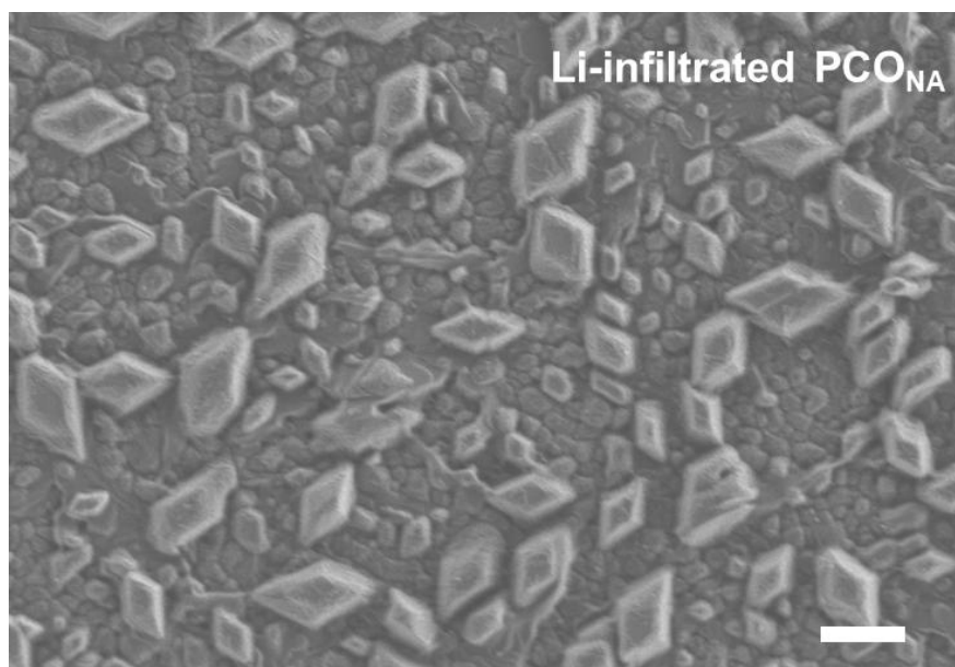
Supplementary Fig. 2 SEM image of Li-infiltrated PCO NA fabricated on Al 2 O 3 . The PCO NA is observed to be fully covered by Li 2 O given infiltration with a concentrated solution. (scale bar, 2 \mu m).
