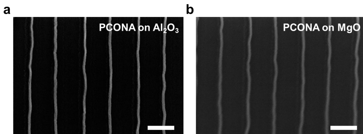
Supplementary Fig. 4 Scanning electron microscopy (SEM) images of PCO NA fabricated on a \text{Al}_2\text{O}_3 and b MgO substrates, respectively (scale bar, 200 nm).
