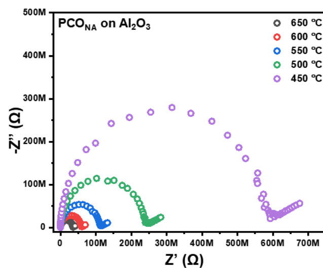
Supplementary Fig. 3 Impedance spectra measured from 450 °C to 650 °C on uninfiltrated PCO NA fabricated on Al 2 O 3 insulating substrate.
