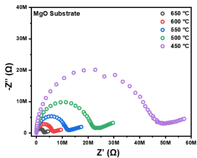
Supplementary Fig. 5 Impedance spectra measured from 450 °C to 650 °C on uninfiltrated PCO NA fabricated on MgO insulating substrate.
