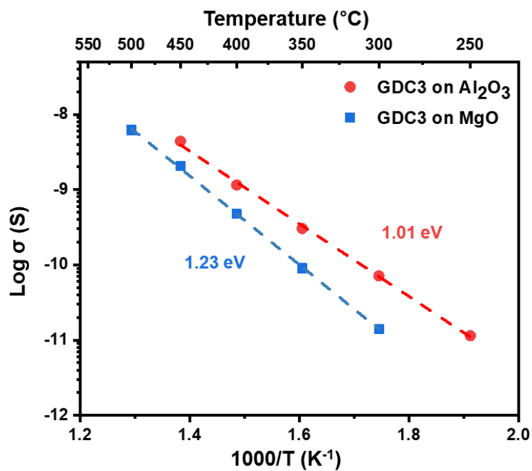
Supplementary Fig. 10 Arrhenius plots of in-plane conductivity of 3 at% Gd-doped ceria (GDC3) nanowire arrays fabricated on \text{Al}_2\text{O}_3 and MgO substrates annealed at 400 ^{\circ}\text{C} along with their respective activation energies.
