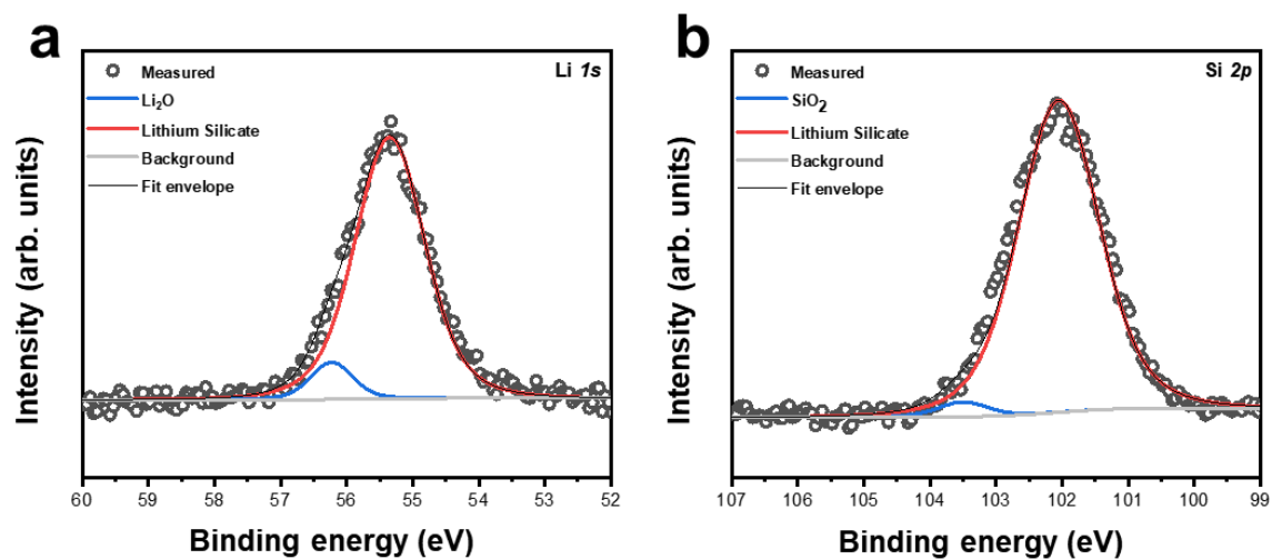
Supplementary Fig. 11 XPS spectra of \text{PCO}_{\text{NA}} after sequential infiltration with Li-species following Si-species, showing the different binding energy regions of Li 1s and Si 2p spectra, respectively.
