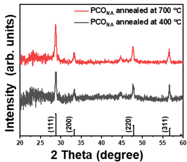
Supplementary Fig. 9 XRD spectra of PCO NA fabricated on Al 2 O 3 substrate annealed at 400 °C and 700 °C, respectively. Black vertical lines at bottom of figure indicate the dominant facets of the cerium oxide crystal structure.
