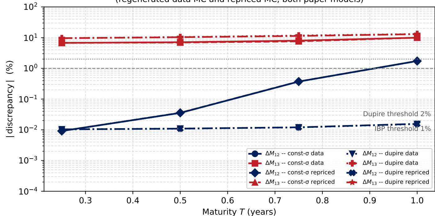
Three-way IBP consistency vs maturity (regenerated data MC and repriced MC, both paper models)
