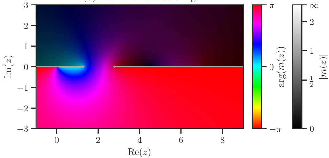
(b) Plain Domain Coloring
