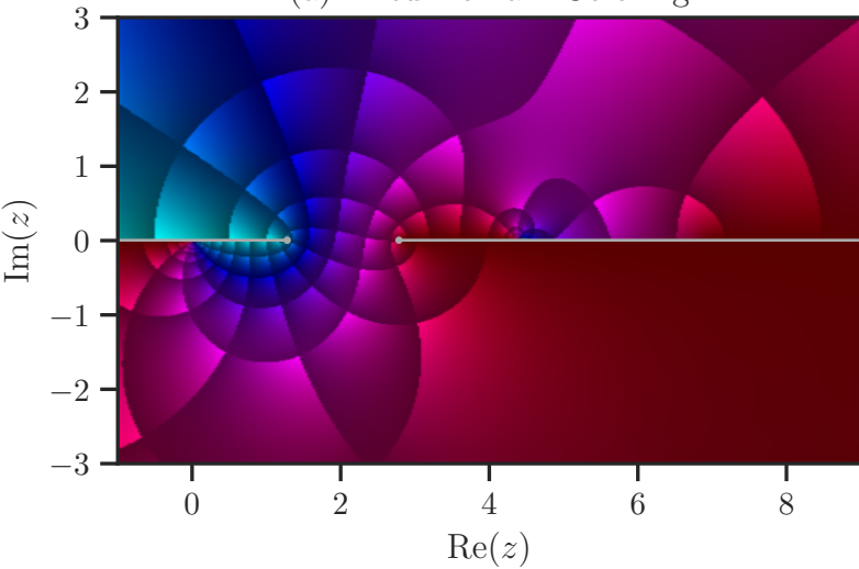
(a) Tiled Domain Coloring
