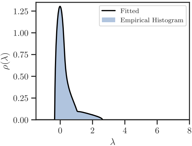
(a) Initial Density ( n = 4K )
