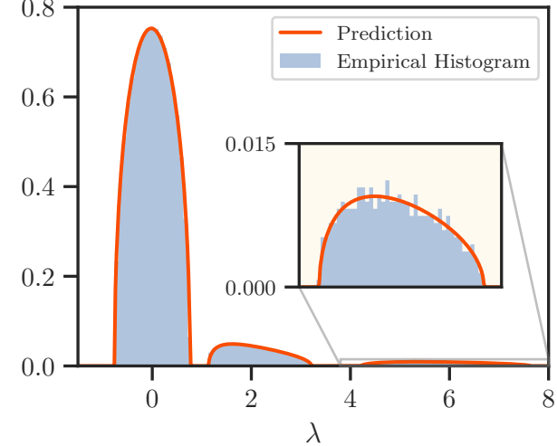
(c) Final Density ( n = 16K )
