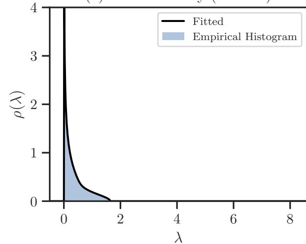
(a) Initial Density ( n = 4\text{K} )
