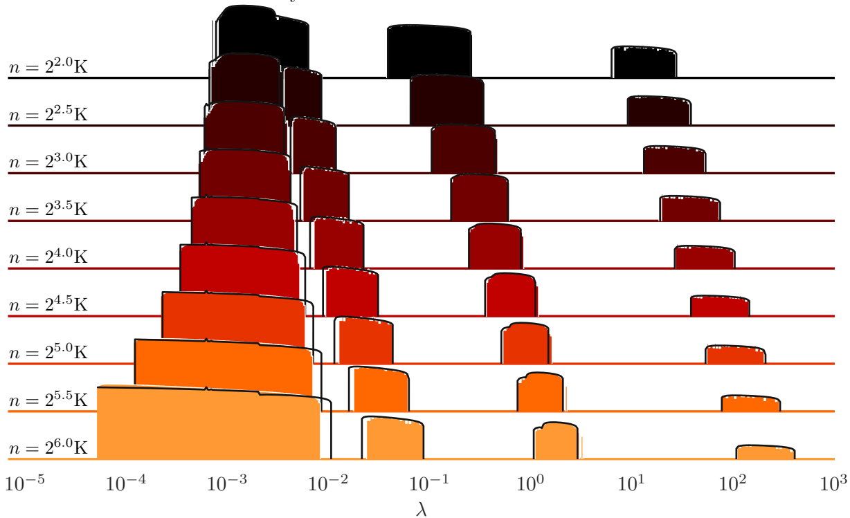
Density evolution from n = 4K to n = 64K
