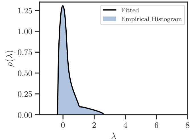
(a) Initial Density ( n = 4\text{K} )
