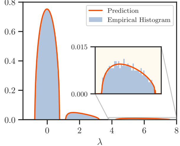
(c) Final Density ( n = 16\text{K} )
