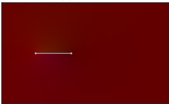
(b) m_2 on \mathbb{C}
