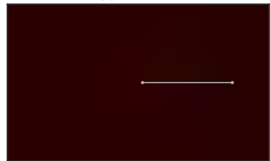
(c) m_3 on \mathbb{C}
