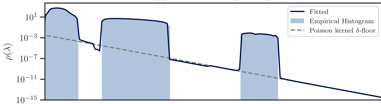
(a) Initial Density ( n = 2K )
