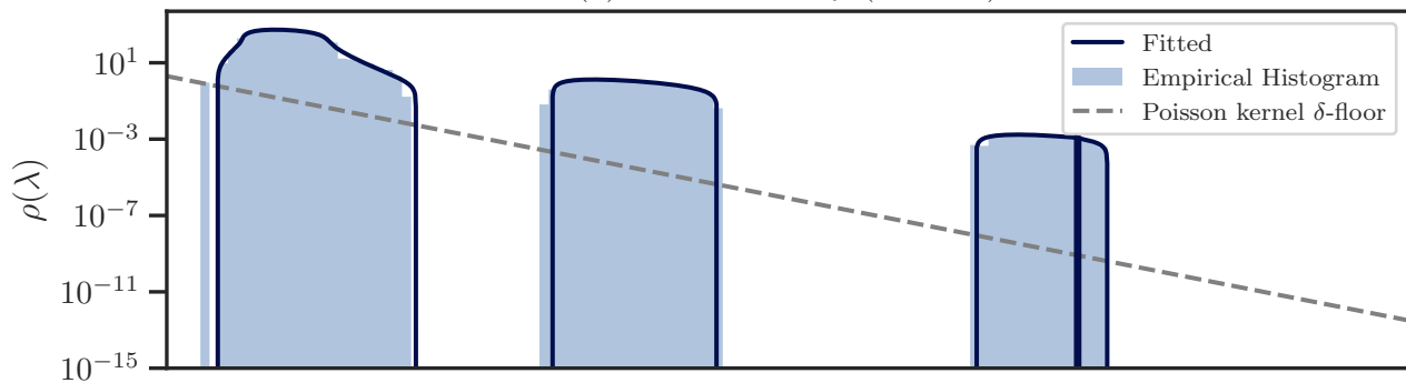
(a) Initial Density ( n = 4K )
