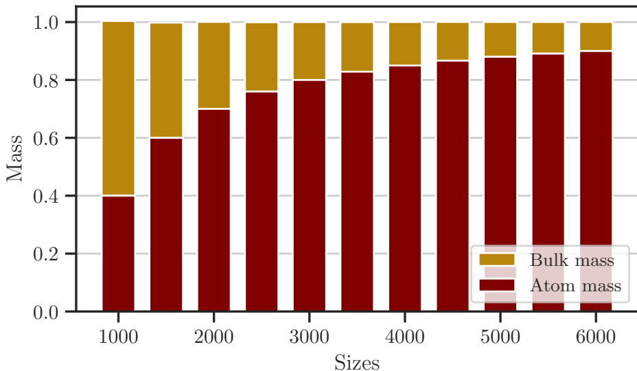
Mass Transfer Between Atoms and Bulks
