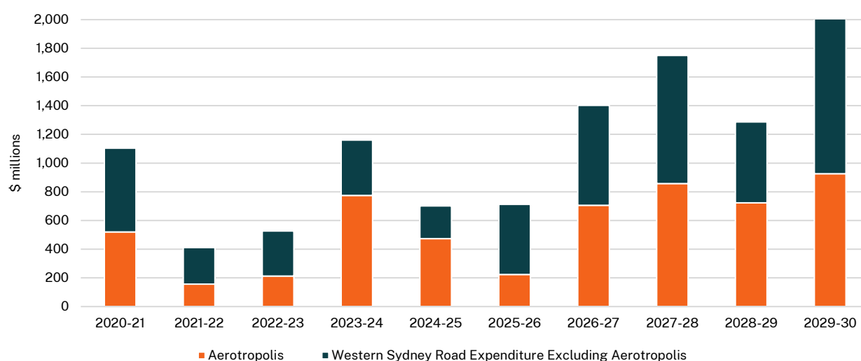
Chart 1.5: Capital expenditure on Western Sydney roads, including Aerotropolis capital expenditure 2020-21 to 2029-30
