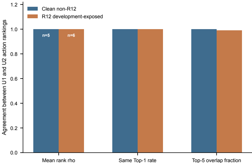
Cost normalization leaves short-horizon ranking nearly unchanged
