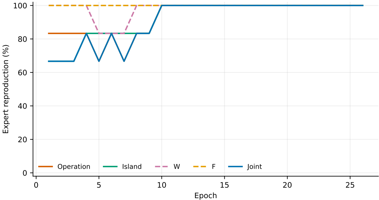
Hard-masked autoregressive imitation accuracy
