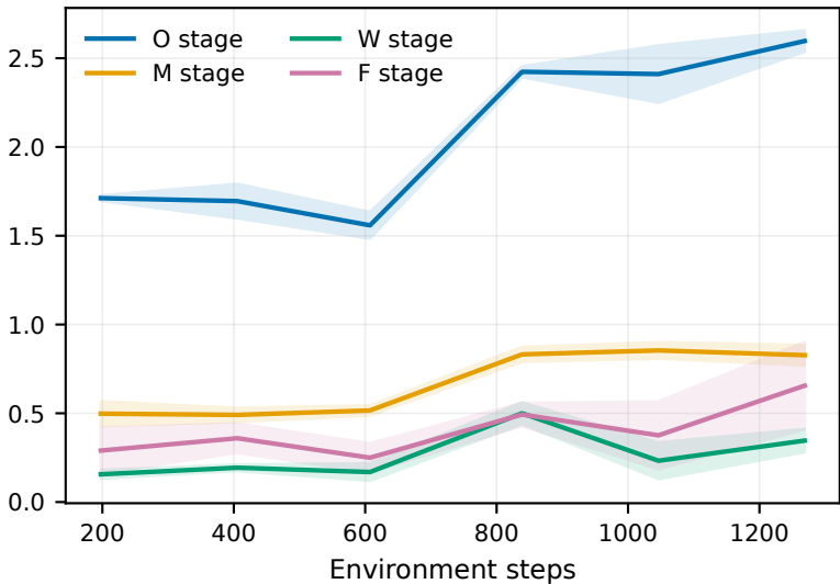
Stage entropy
