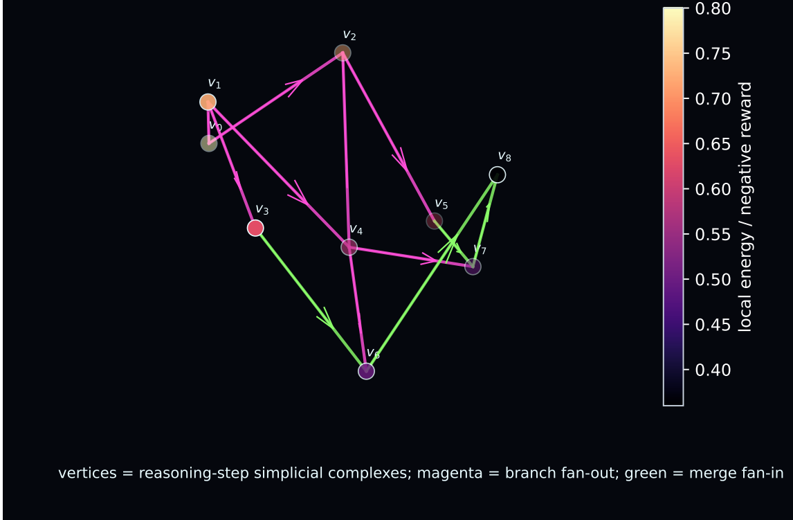
Figure 6: Graph-of-thought trajectory as a branch/merge DAG. Reasoning vertices carry local simplicial complexes and hidden-state certificates; branch fan-out explores alternatives and merge fan-in reconciles them.
