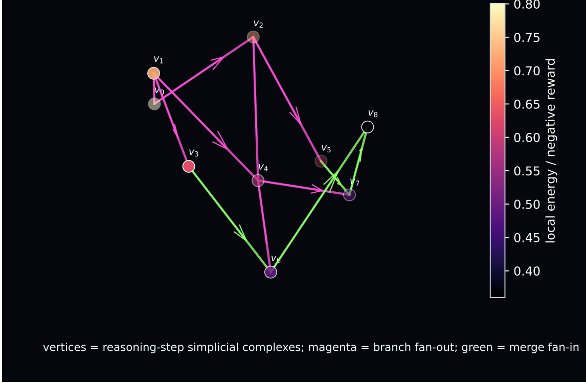
Figure 6: Graph-of-thought trajectory as a branch/merge DAG. Reasoning vertices carry local simplicial complexes and hidden-state certificates; branch fan-out explores alternatives and merge fan-in reconciles them.
