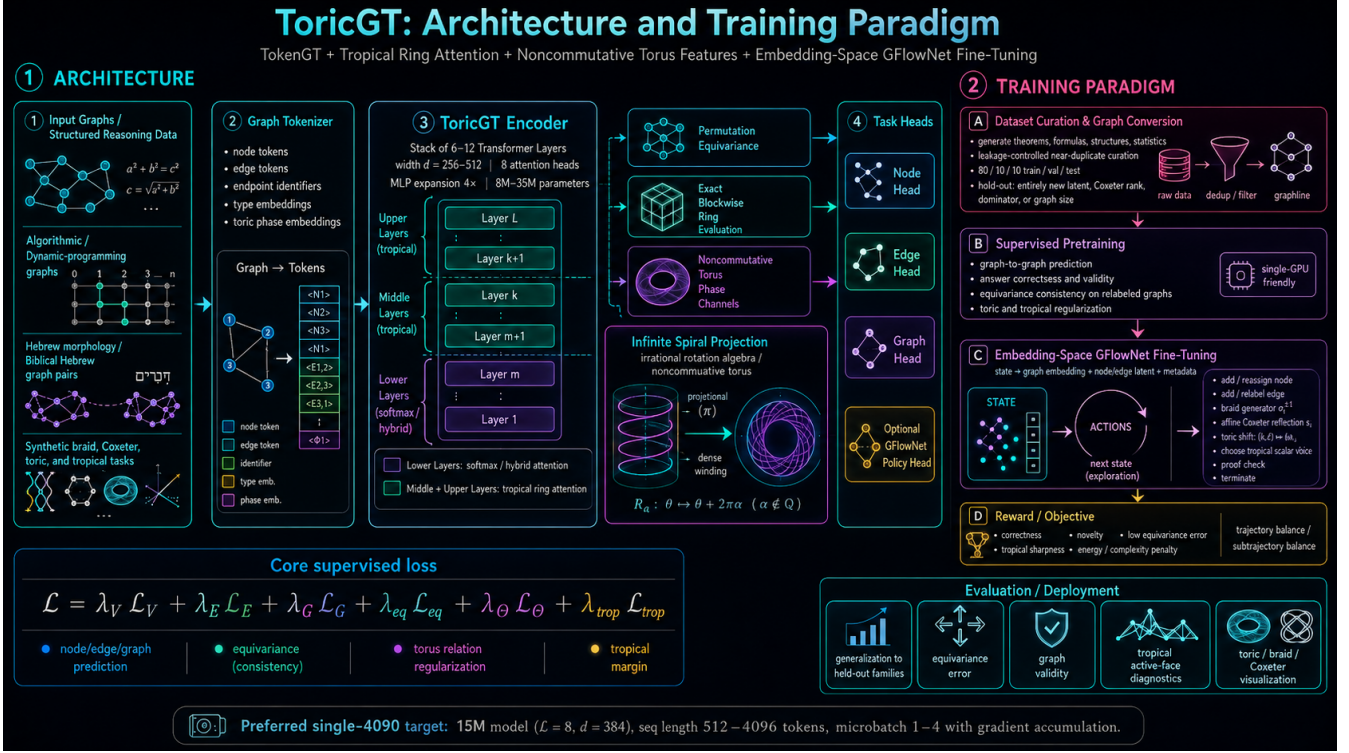
Figure 1: ToricGT combines graph tokenization, tropical ring attention, noncommutative-torus phase channels, Soft-MoE routing, embedding-space GFlowNet fine-tuning, and training-only Forest-of-Thought search.
