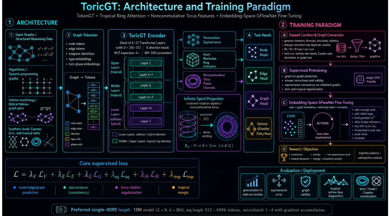
Figure 1: ToricGT architecture and training program. Typed graph tokens carry node, edge, end-point, structural, tropical, toric phase, and optional BGG-certificate features. The encoder combines ordinary attention, tropical ring attention, Soft-MoE adapters, and low-rank certificate probes. Training combines supervised graph losses, BPB or language-model loss, GFlowNet trajectory balance, GraphCG disentanglement, and Toric BGG homological consistency.
