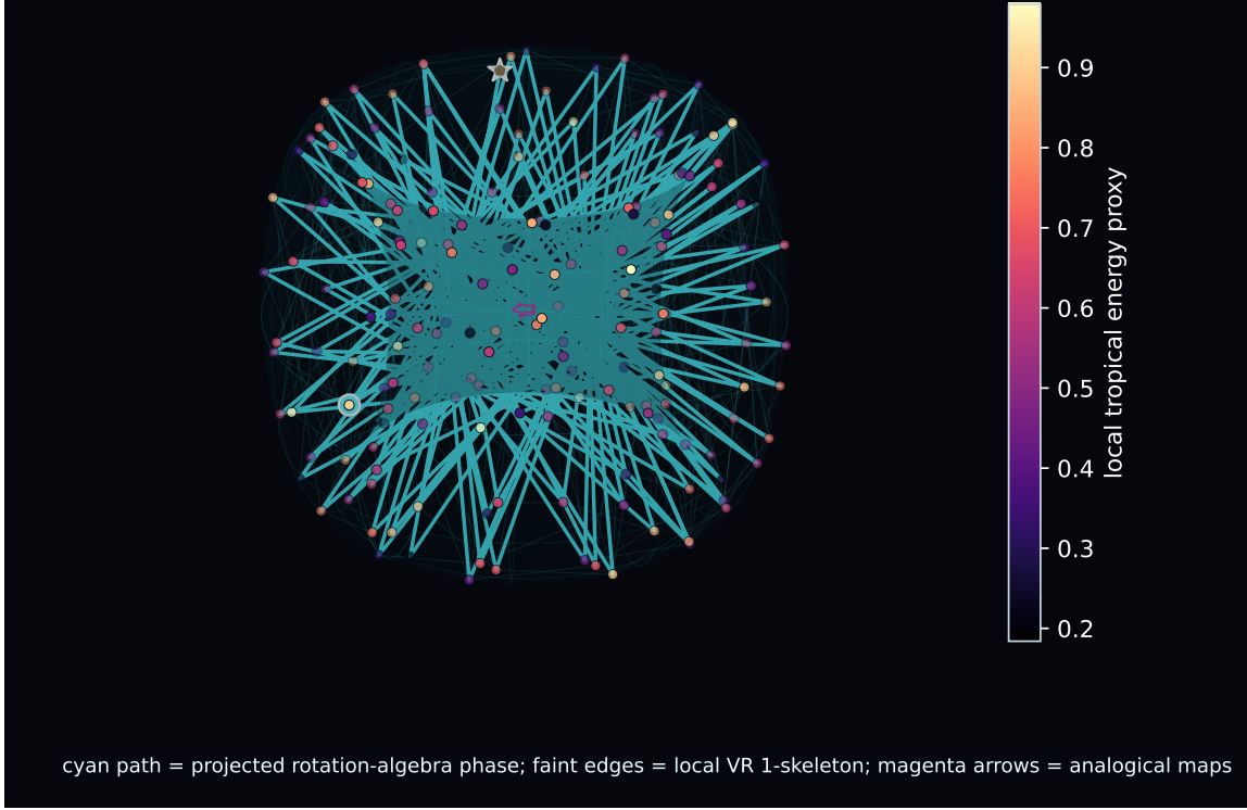
Figure 5: Irrational toric phase projection of a reasoning trajectory. The torus path shows pseudo-periodic phase coverage; faint local edges are Vietoris–Rips 1-simplices; magenta arrows represent window-to-window analogical maps.
