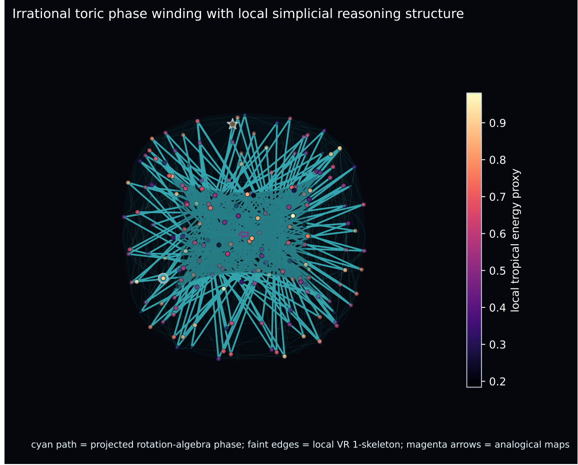
Figure 4: Irrational toric phase projection of a reasoning trajectory. The torus path shows pseudo-periodic phase coverage; faint local edges are Vietoris–Rips 1-simplices; magenta arrows represent window-to-window analogical maps.
