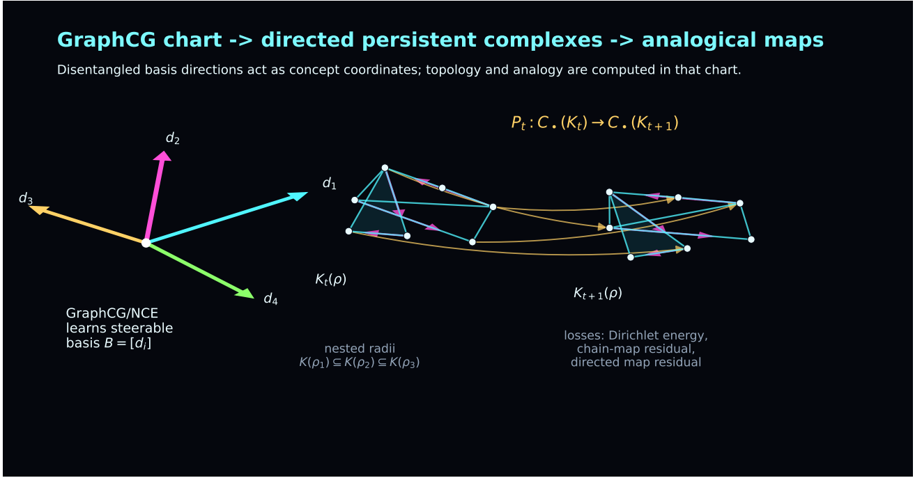
Figure 3: GraphCG supplies a steerable concept chart; ToricGT builds directed persistent complexes in that chart and learns soft functor-like maps that also preserve filtered topological structure.
