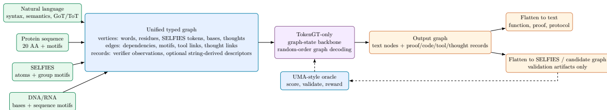
Figure 11: High-level graph-state architecture. Early training uses text, SELFIES/SMILES, protein/DNA/RNA sequences, proof/code/tool traces, and thought graphs. Actual structure files and dynamics trajectories are not training inputs; UMA-style systems are external oracles for validation and reward.
