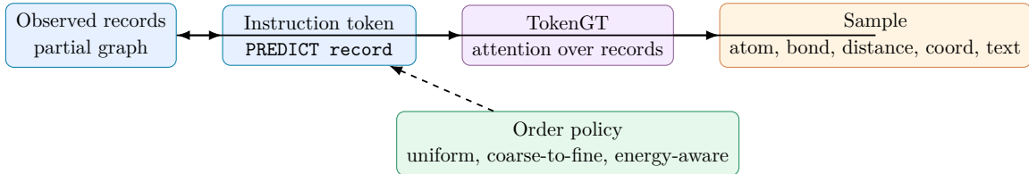
Figure 12: Random-order graph-to-graph autoregression. The next output record may be a SELF-IES token, residue token, motif token, claim node, thought node, tool result, verifier result, UMA-oracle score, or repair action, always conditioned on the input graph and the partial output graph.
