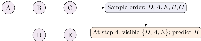
Figure 10: Random-order graph autoregression. The graph has structural edges independent of the reveal order. Training samples many reveal orders so the model learns to complete partial relational objects.
