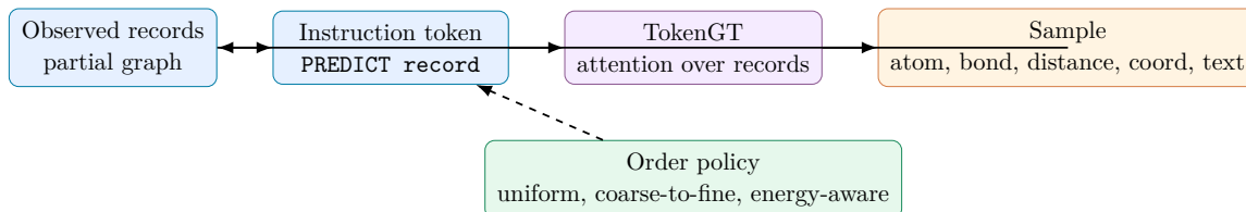
Figure 13: Random-order graph-to-graph autoregression. The next output record may be a SELF-IES token, residue token, motif token, claim node, thought node, tool result, verifier result, UMA-oracle score, or repair action, always conditioned on the input graph and the partial output graph.
