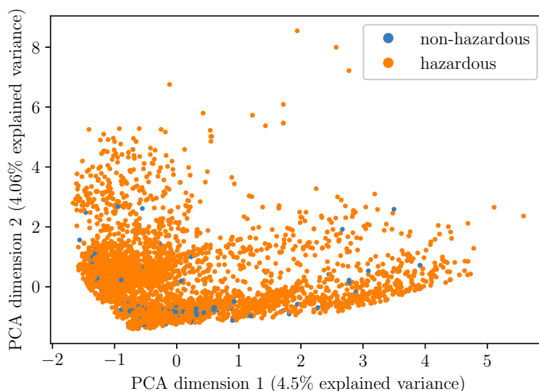
Figure 2: Two-dimensional principal component analysis of dataset represented as molecular fingerprints, explaining 8.56% of total variance.
