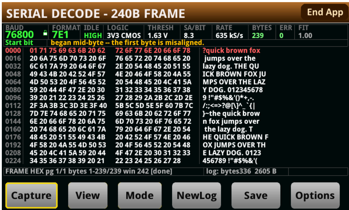
Figure 3: One misaligned byte: ERR reads 0, the row is red, the note names it
