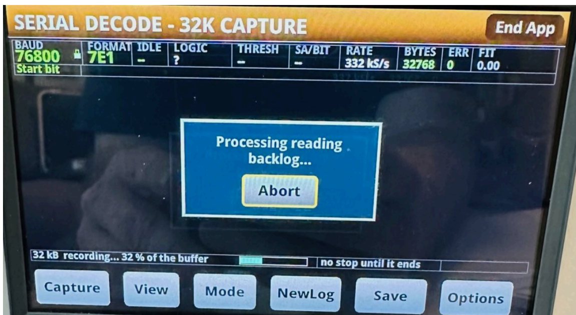
Figure 9: The instrument's own backlog dialog, over a 32 kB recording at 76.8 kBd
